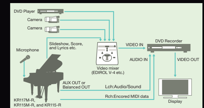
▲ Setup Example
