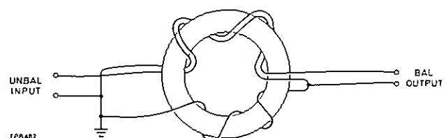
WIRING DIAGRAM
