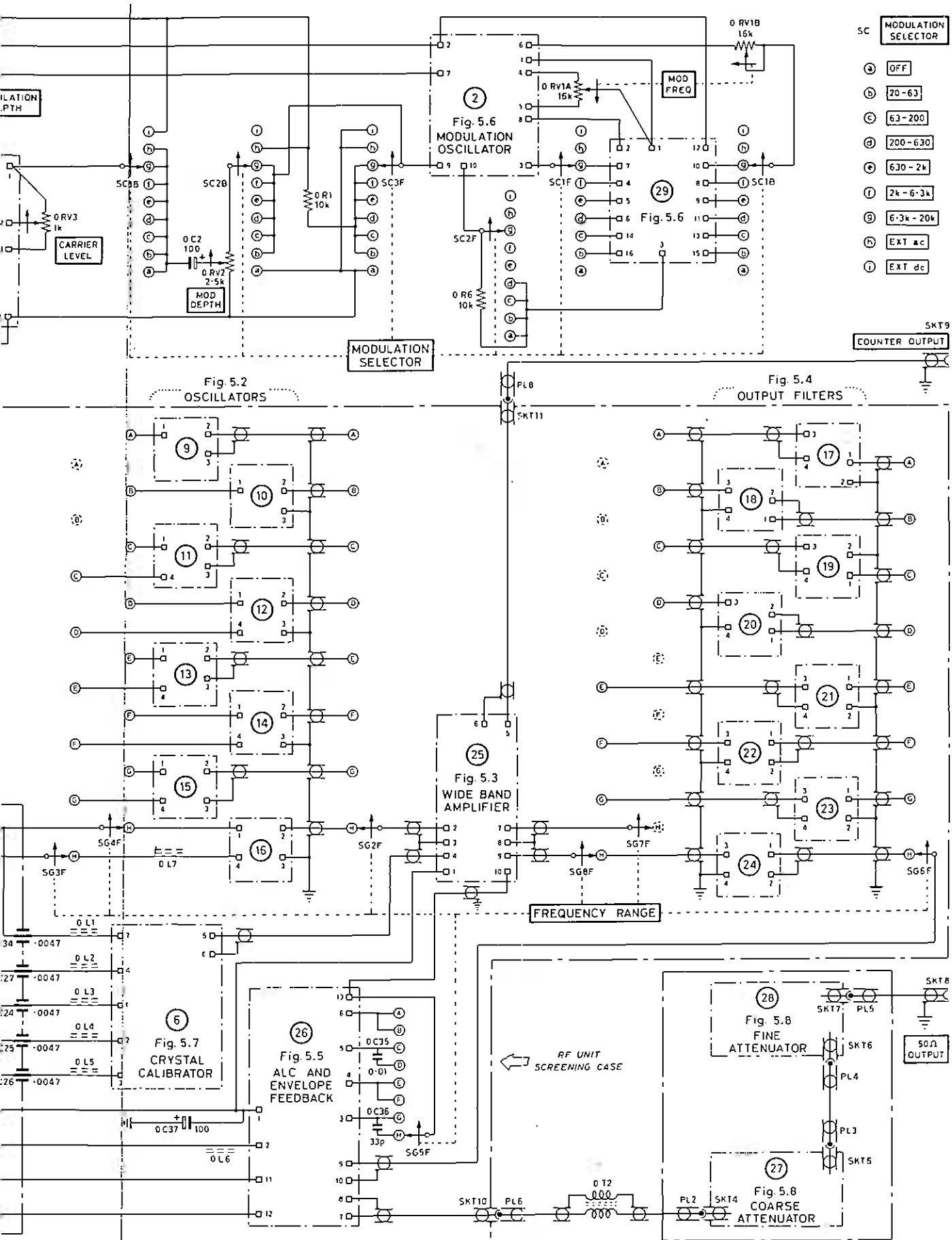
Fig. 5.1 Interconnection diagram
