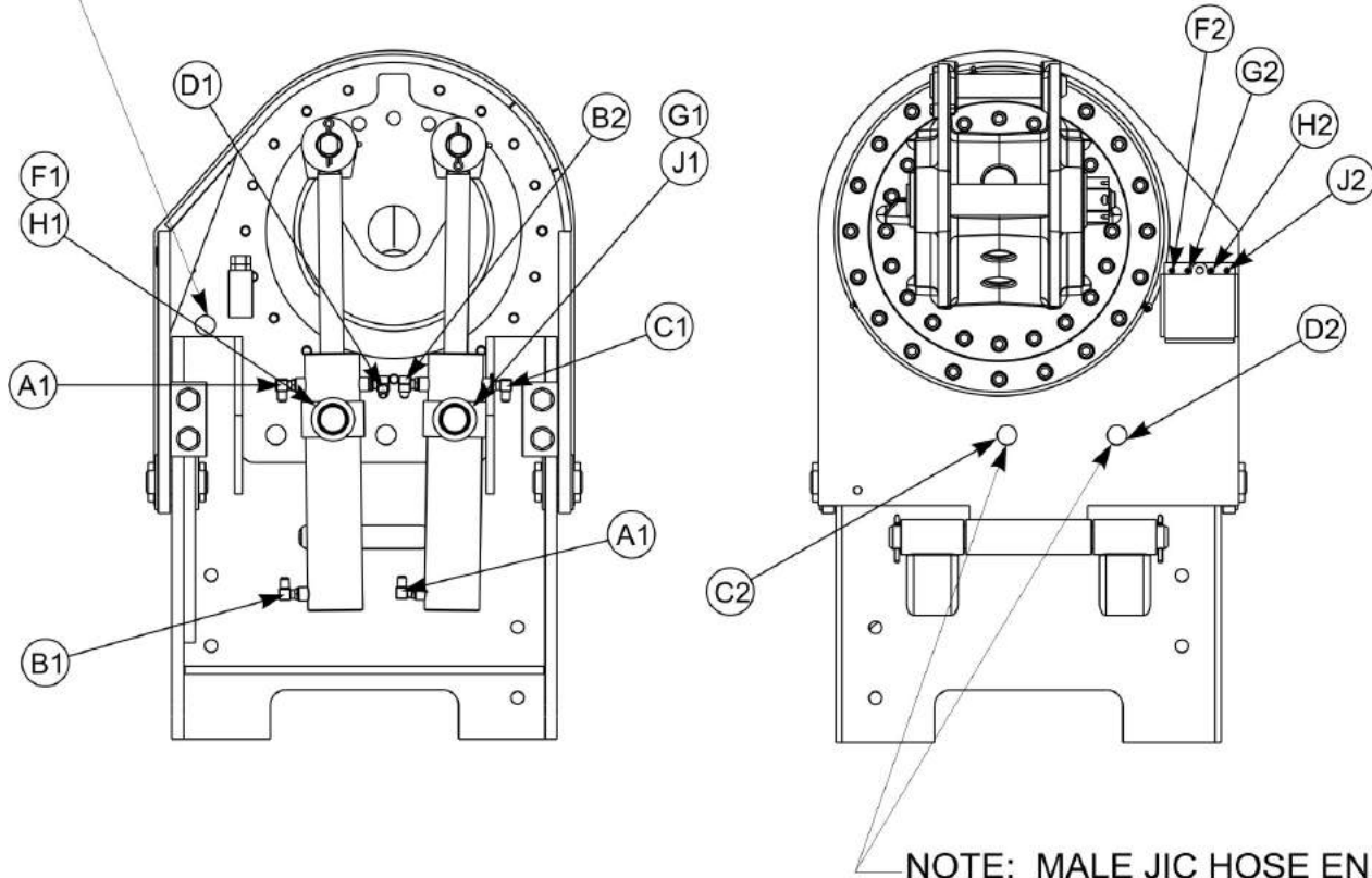
HOSE ROUTING CHART
