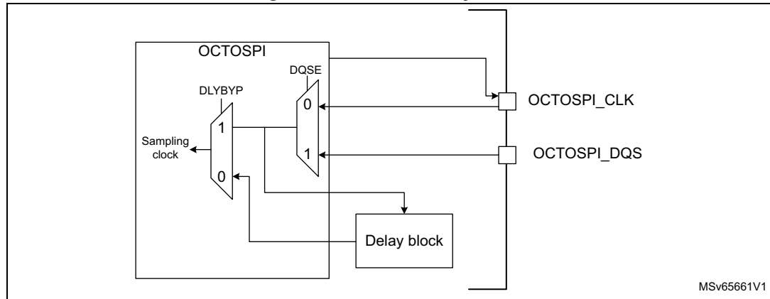
Figure 5. OCTOSPI delay block
