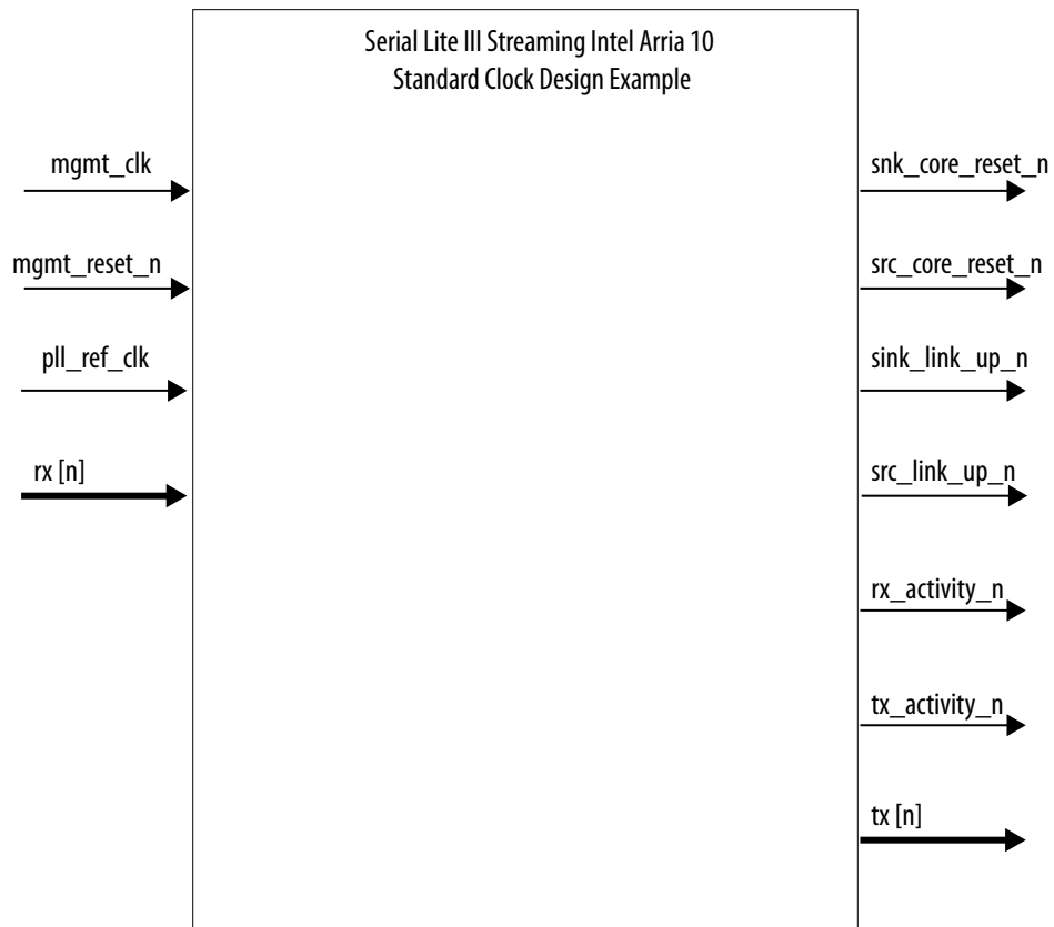
Figure 15. Top-level Signals for Intel Arria 10 Serial Lite III Streaming Standard Clocking Mode Design Example
