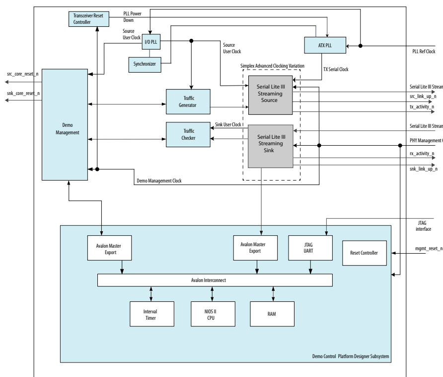
Figure 16. Design Example for Simplex Core in Advanced Clocking Mode
