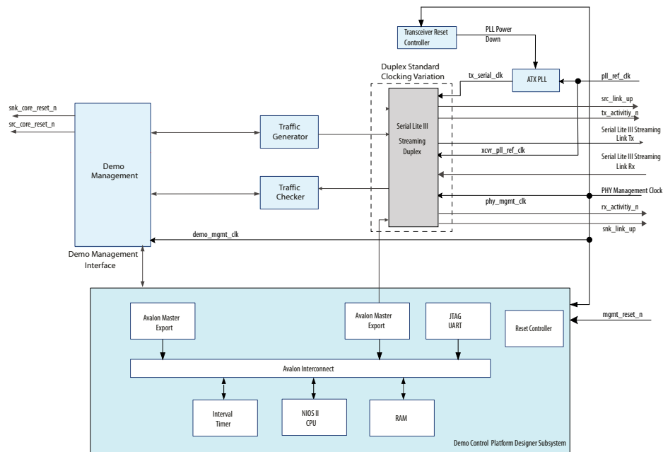
Design Example for Duplex Core in Standard Clocking Mode
