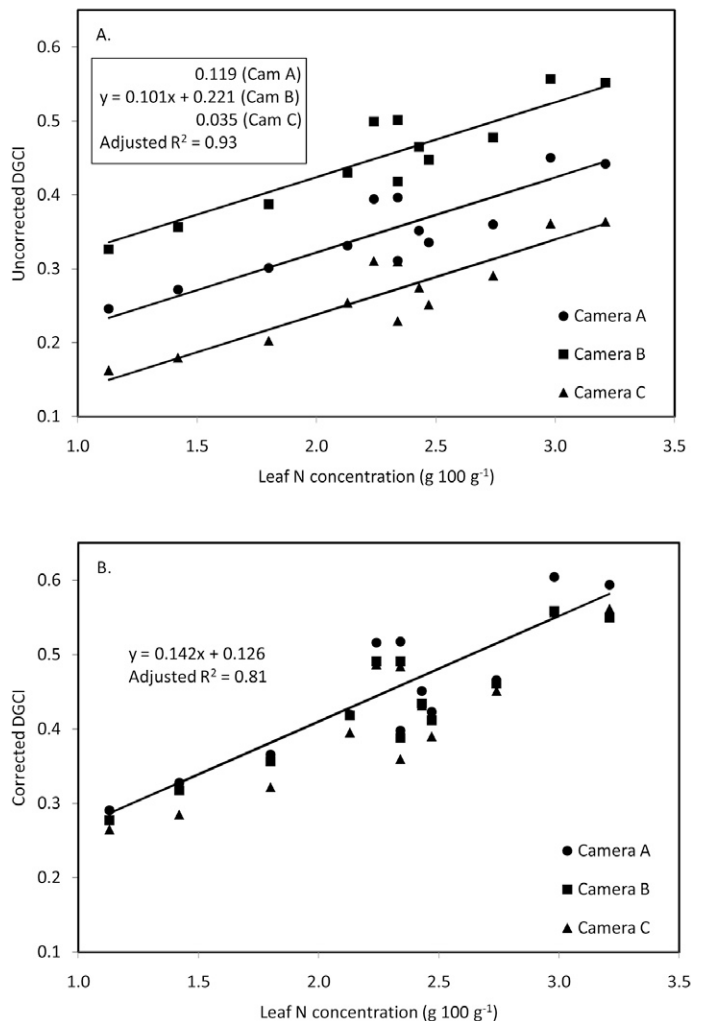
Figure 3. Uncorrected dark green color index (DGCI) values for three cameras versus leaf N concentration (Panel A). Corrected DGCI values versus leaf N concentration (Panel B). Cameras were used as covariates to determine if there were statistical differences in slope and intercept before and after correction with calibration disks.
