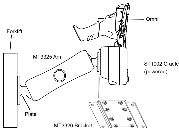
Figure 4-18 MT3325 Standard Arm Kit with Omnii Vehicle Cradle Clamp and Rail Bases (Torque to 26 in-lbs)
