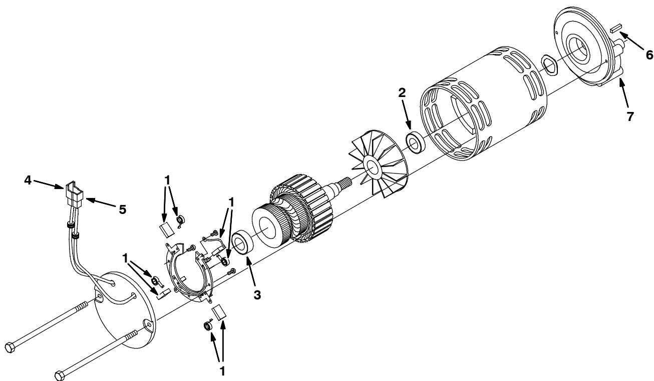
Fig. 10 - Electric Motor Breakdown, 222255AM
