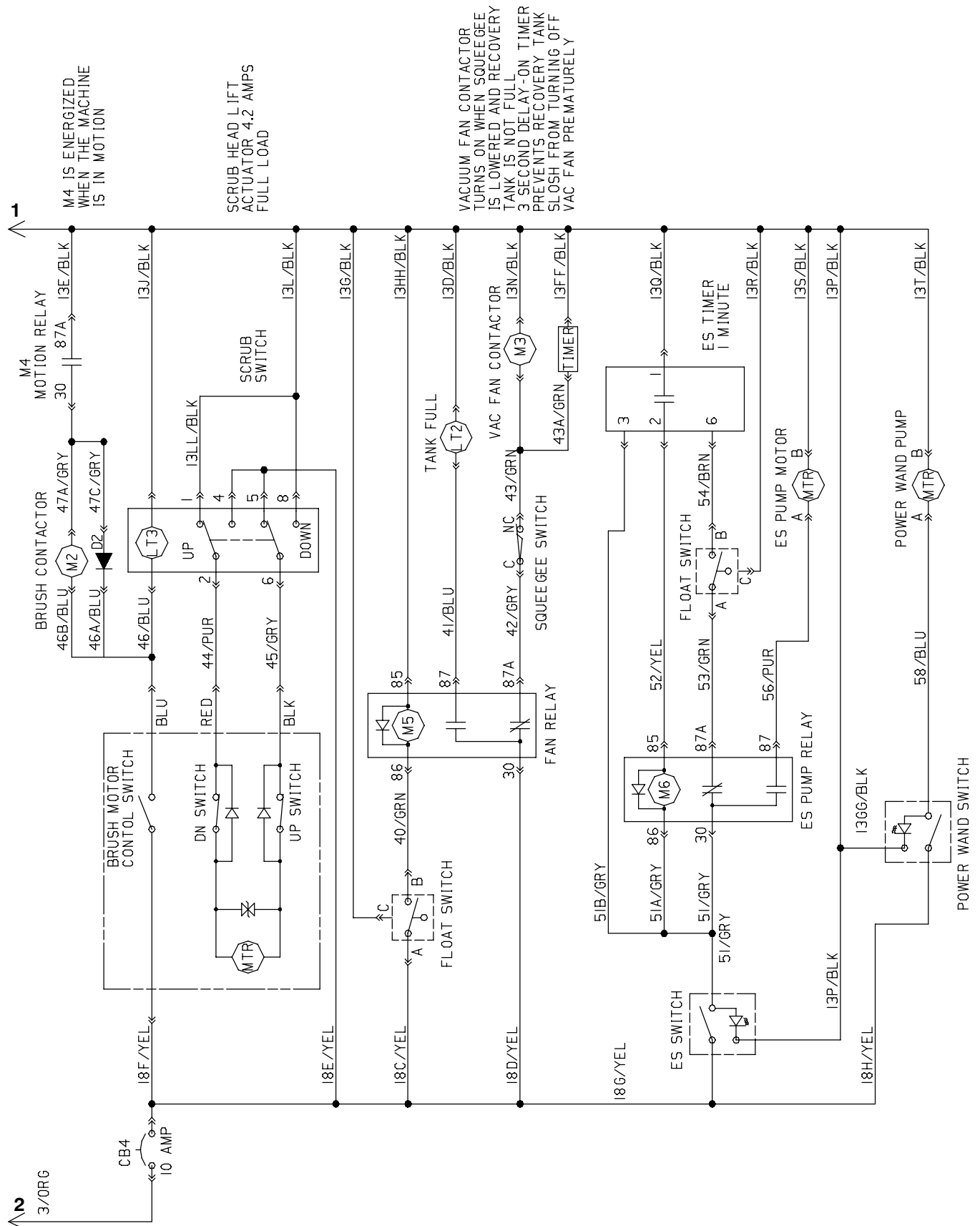
Fig. 36 - Electrical Schematic (022000- )
