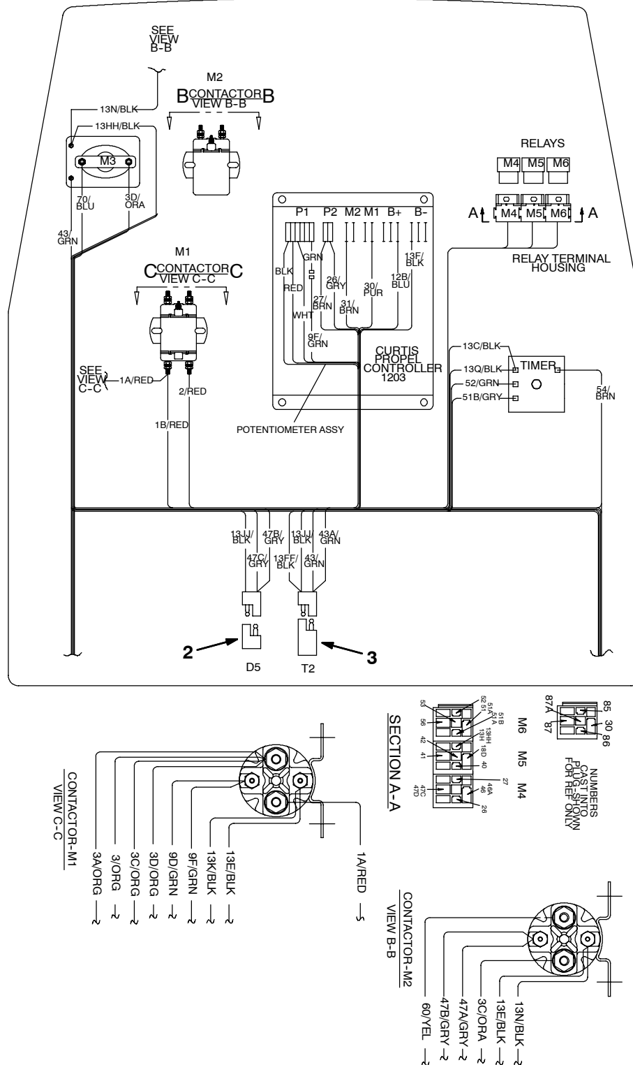
Fig. 37 - Electrical Wire Harness Group (000000-021999)
