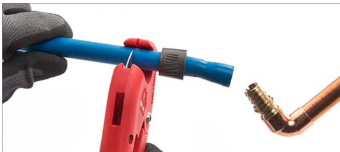
Fig. 4.13: Cut off 3 in. of pipe from end prior to making new joint
