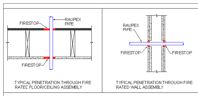
Fig. 5.5: RAUPEX pipe is fire-stopped at both points of entry through the assembly
