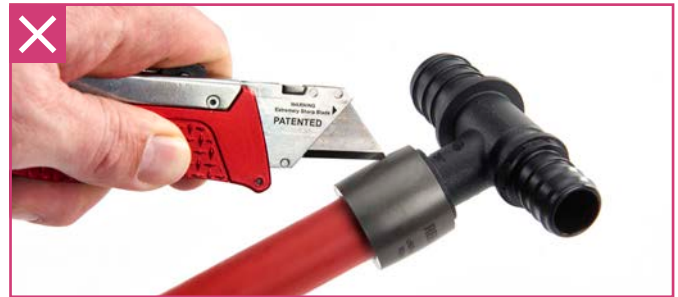
Fig. 4.9: DO NOT cut the EVERLOC+ compression sleeve from finished joint
