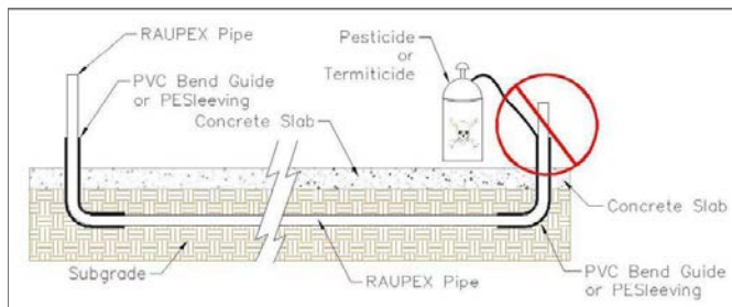
Fig 6.9: Slab penetration protection
