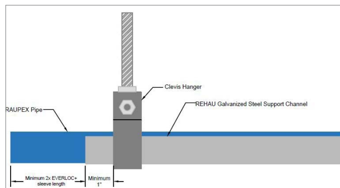
Fig. 6.18: RAUPEX pipe supported with steel support channel
