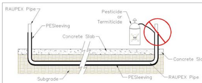
Fig. 6.8: Continuous sleeve installation
