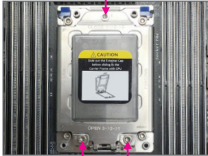
Screw 3 Screw 2
