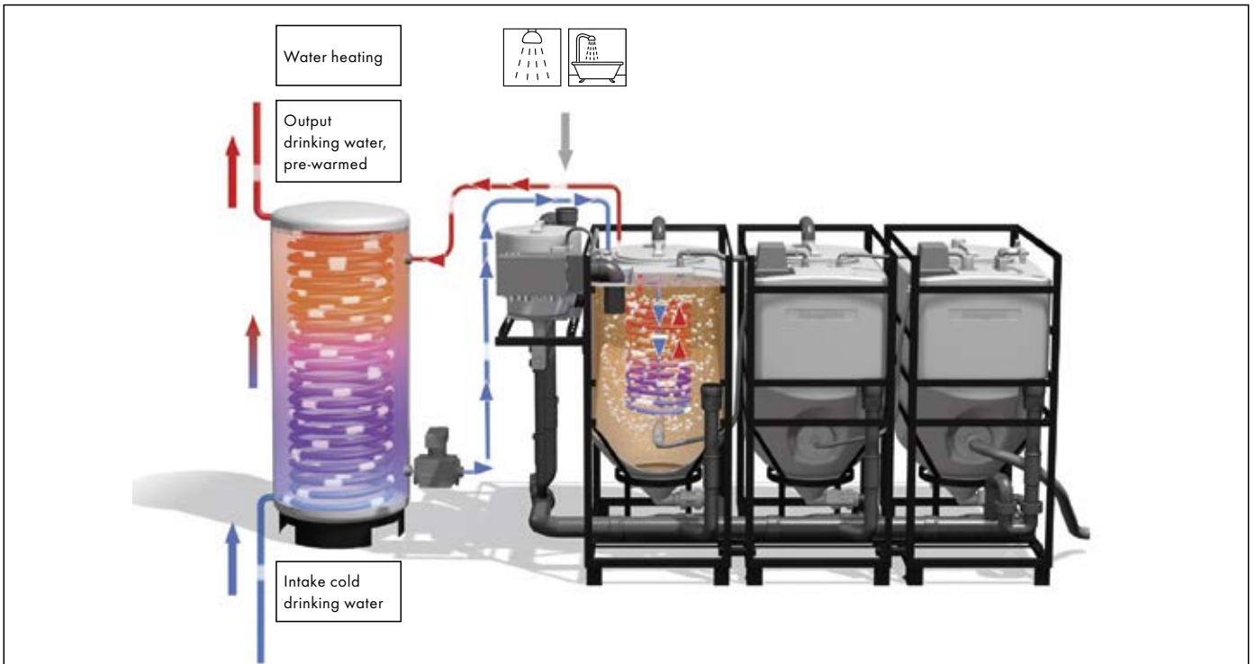
Pontos HeatCycle technology.
