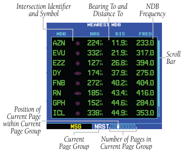
Figure 7-10 Nearest NDB Page
