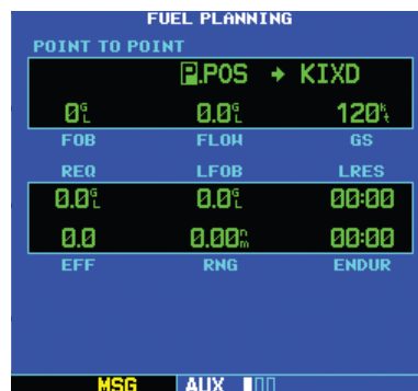
Figure 8-6 Fuel Planning Page, Point-to-Point
