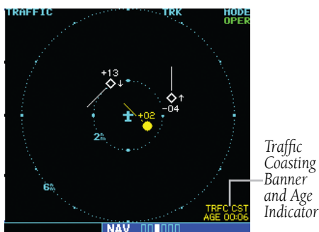
Figure 12-6 Traffic Age Indicator and Coasting Banner
