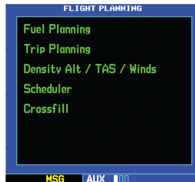
Figure 8-3 Flight Planning Page
