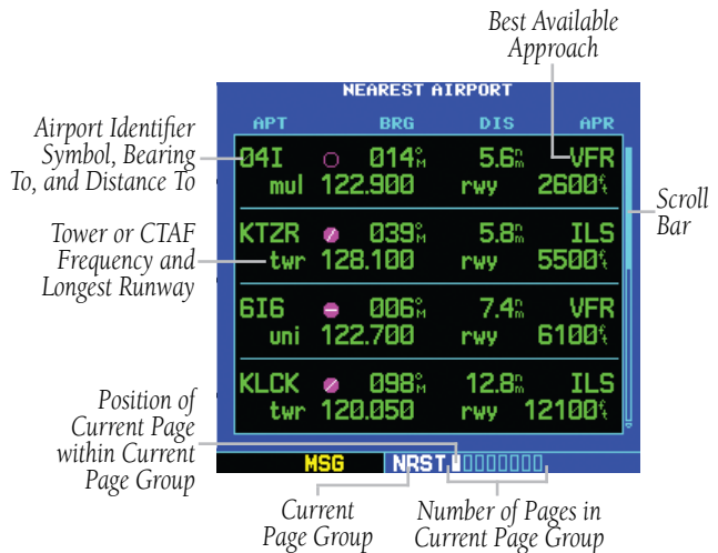
Figure 7-6 Nearest Airport Page
