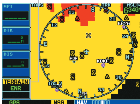
Figure 11-2 TAWS Annunciation Field
