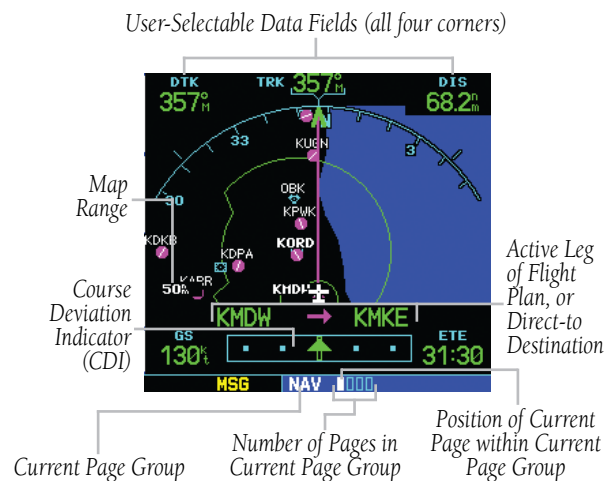
Figure 2-4 Default NAV Page
