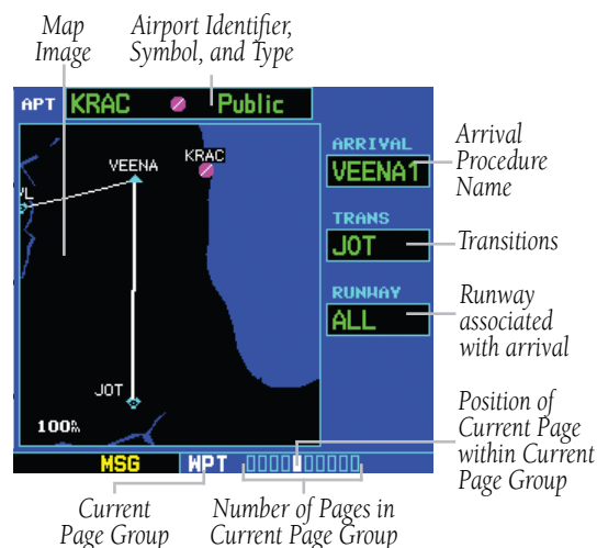
Figure 6-22 Airport Arrival Page
