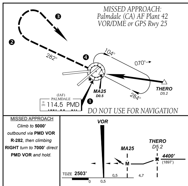
Figure 5-53 Palmdale Missed Approach
