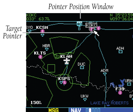
Figure 2-12 Panning on Map Page
