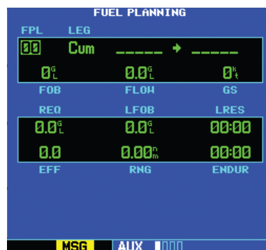
Figure 8-7 Fuel Planning Page, Flight Plan
