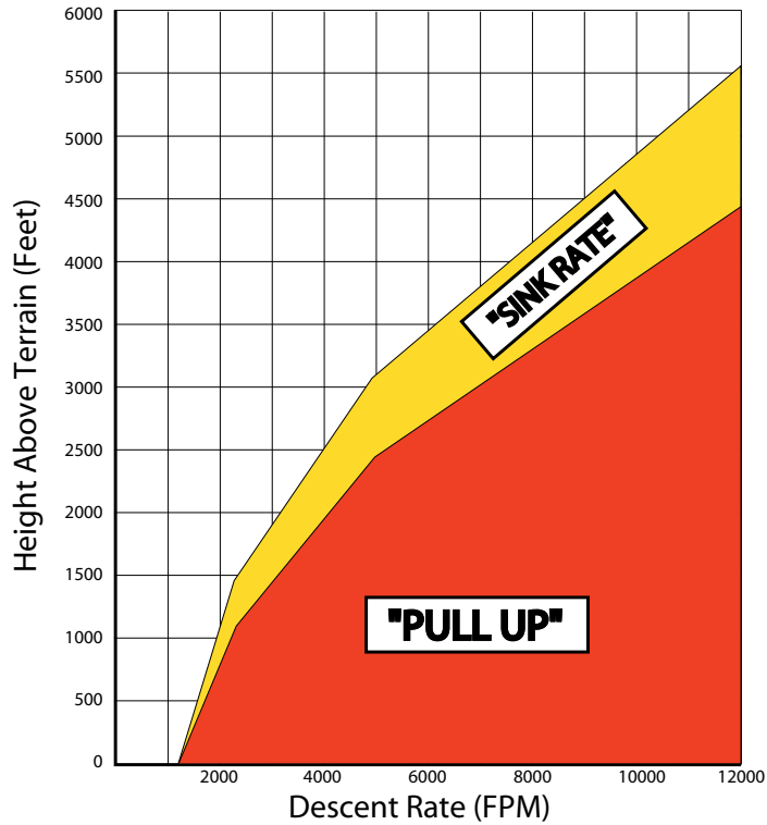
Figure 11-8 Excessive Descent Rate Alert Criteria
