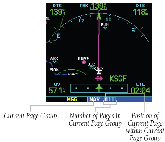
Figure 1-12 Current Page and Page Group
