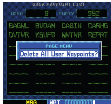
Figure 6-48 User Waypoint List Page Menu
