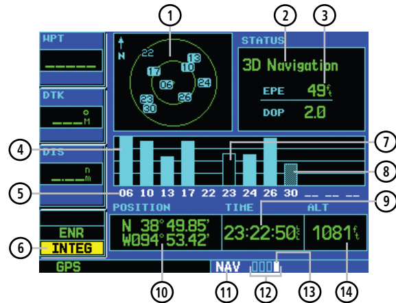
Figure 2-47 Satellite Status Page
