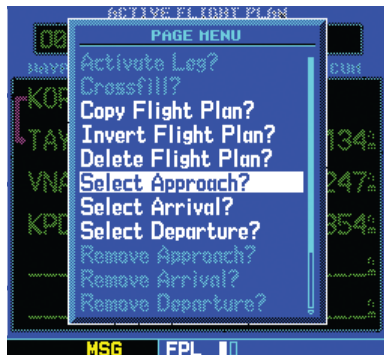
Figure 4-23 Active Flight Plan Page Menu
