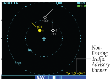
Figure 12-14 Non-Bearing TA Banner
