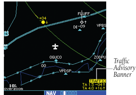
Figure 12-15 Map Page Displaying Traffic
