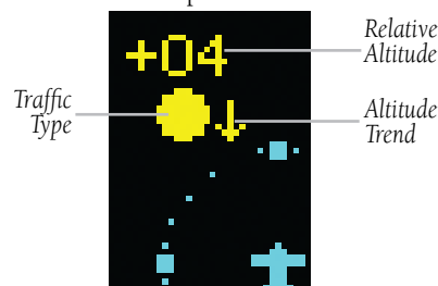
Figure 12-19 Traffic Symbol Components
