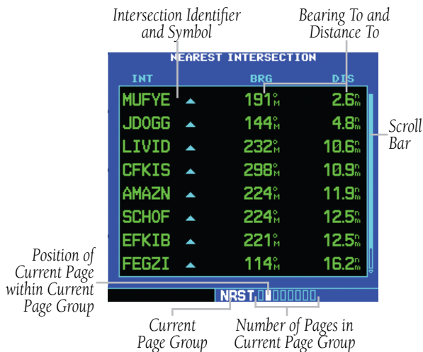
Figure 7-9 Nearest Intersection Page
