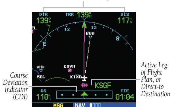
Figure 1-16 Default NAV Page
