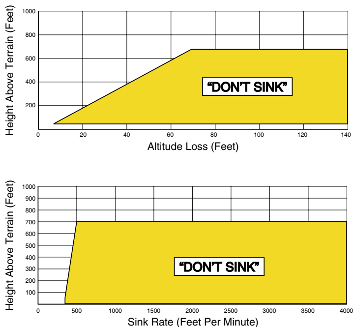
Figure 11-9 Negative Climb Rate (NCR) Alert Criteria
