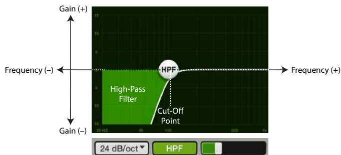
HPF ON at a 24 dB/oct slope
