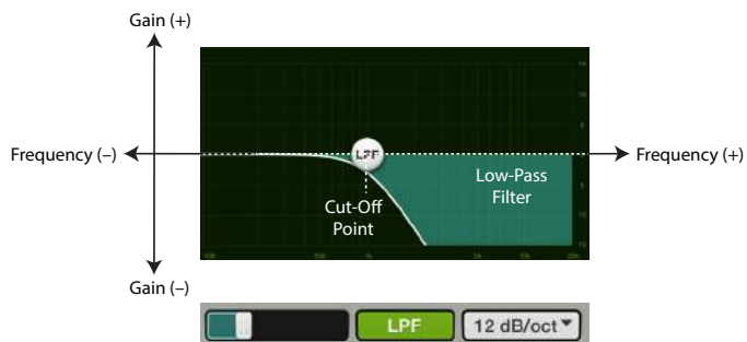
LPF ON at a 12 dB/oct slope
