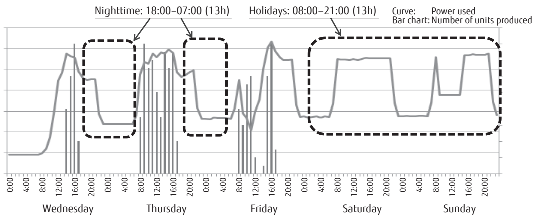
Figure 6 Standby power visualization results.
