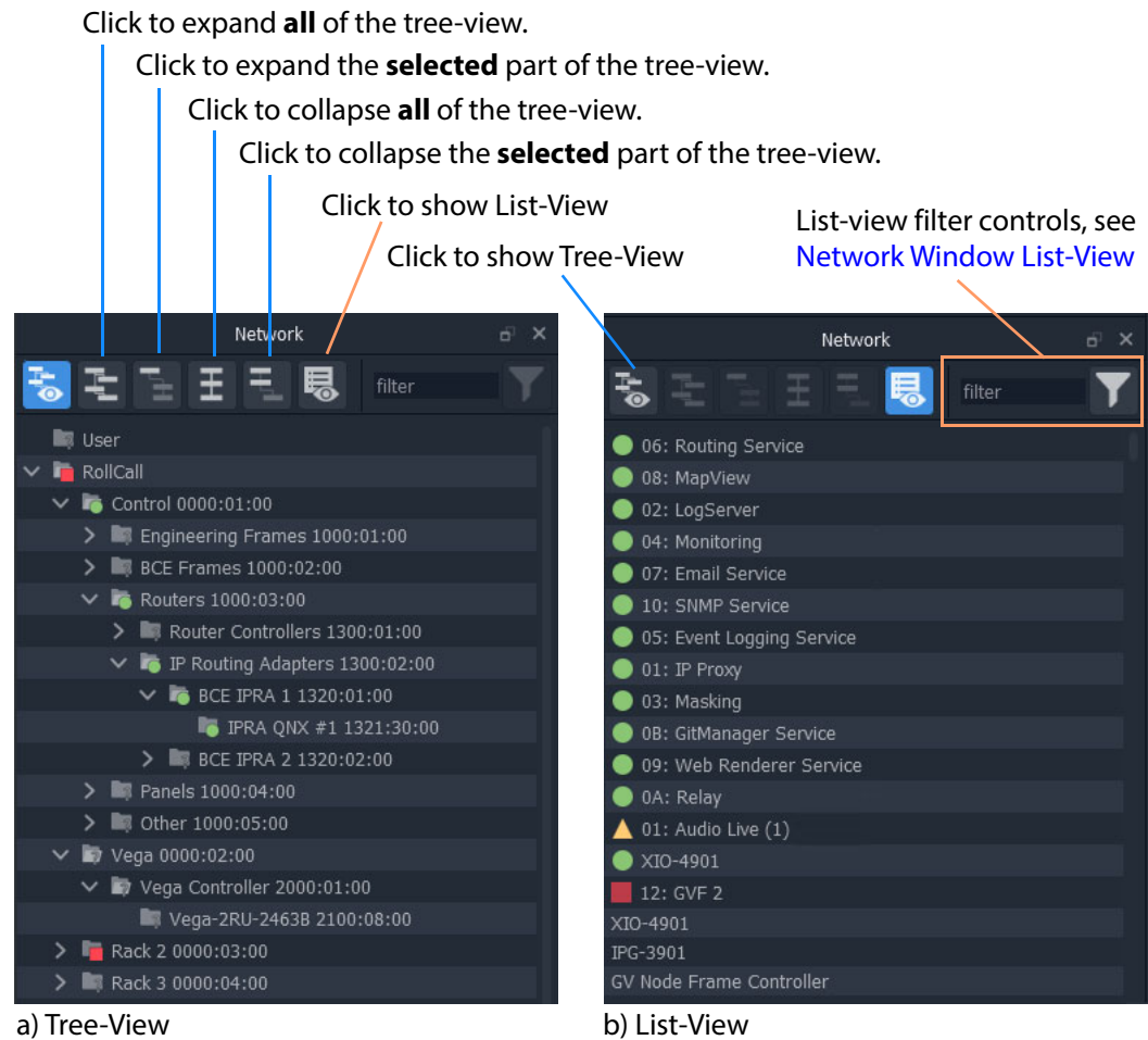
Fig. 3-8: Network Window: a) Tree-View; b) List-View.
