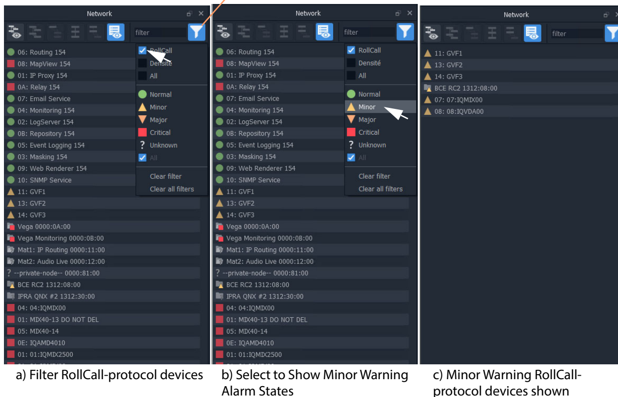
Fig. 3-11: Filter on Device Type and then Alarm State
