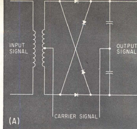
RING (A), dual-control pentode (B)
