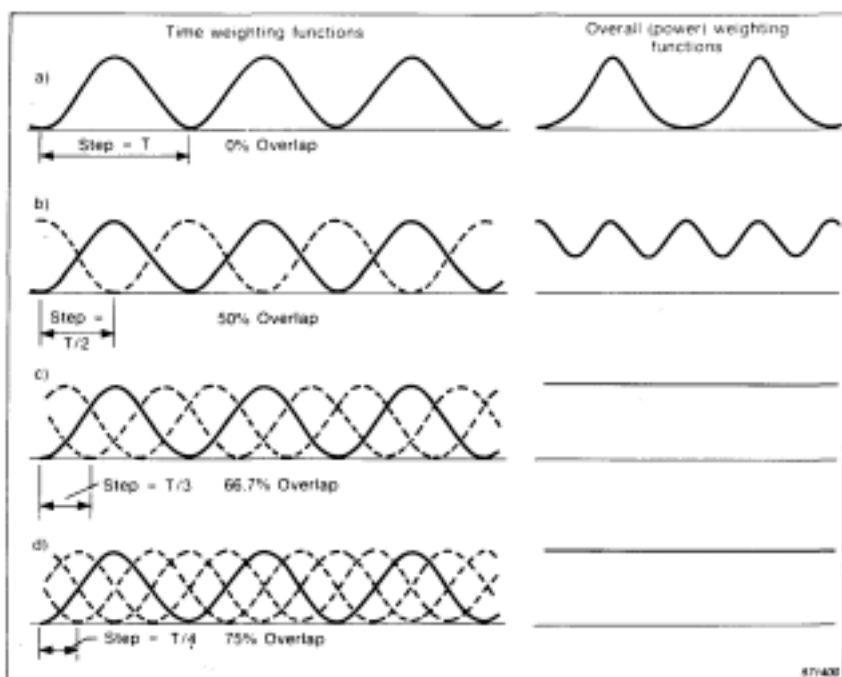
Fig. C.4. Overall weighting functions for overlapping Hanning windows
