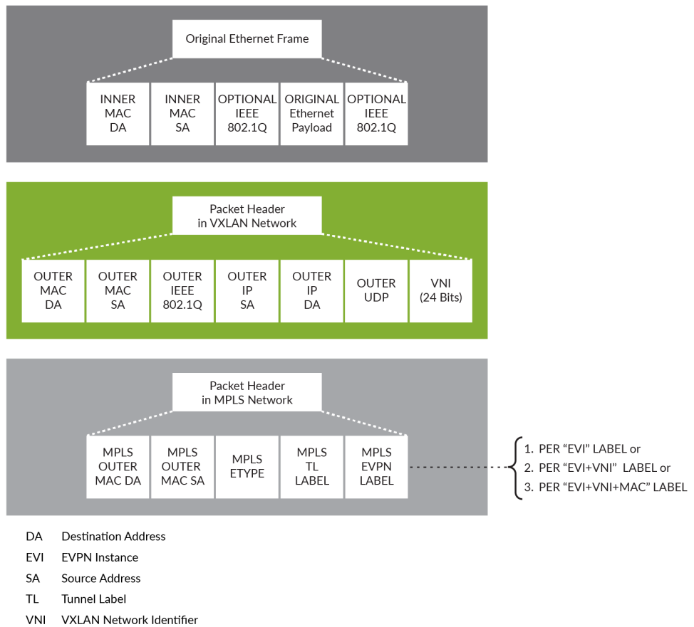
Figure A.1 Difference between Ethernet Frame, VXLAN Header, and, for Reference, the MPLS Header
