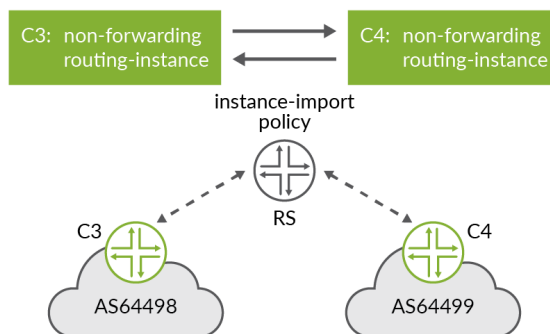
Figure 1.6 Junos Loc-RIB Implementation
