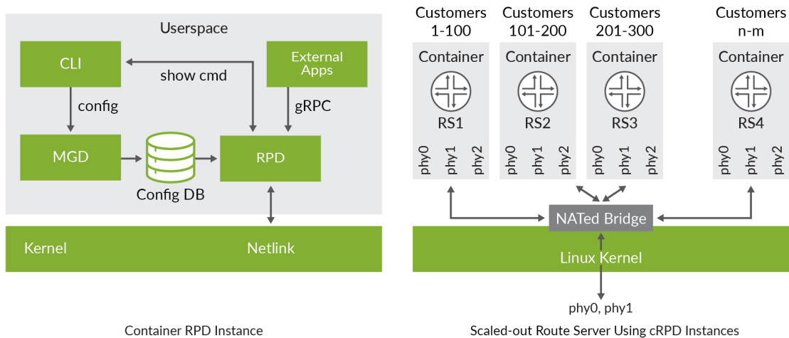
Figure 2.3 cRPD and cRPD as a Scaled-out Route Server
