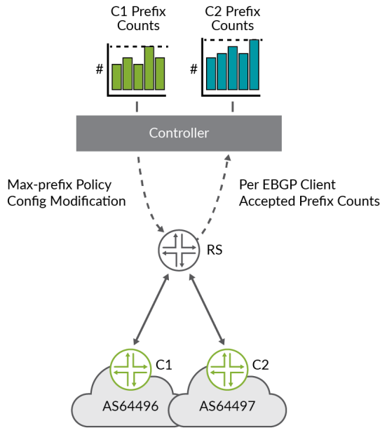
Route Server With Controller Based Dynamic Maximum Prefix Computation
