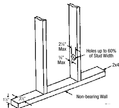
Figure 4.5 Holes in Non-Bearing Walls
