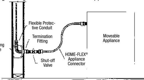
Figure 4.16 HOME-FLEX® Connection to Moveable Gas Appliance
