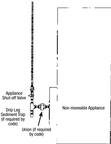
Figure 4.15 Direct Connection to Fixed Appliance
