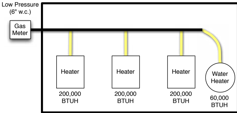
Figure 3.9 Low Pressure Hybrid System—Series Arrangement
