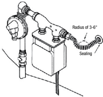
Figure 4.14 Independently Supported Meter
