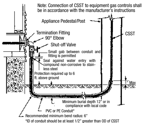
Figure 4.20 Fixed Outdoor Appliance (Underground Routing)
