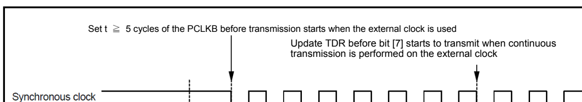
Figure 25.77 Restrictions on the use of external clock in clock synchronous transmission
