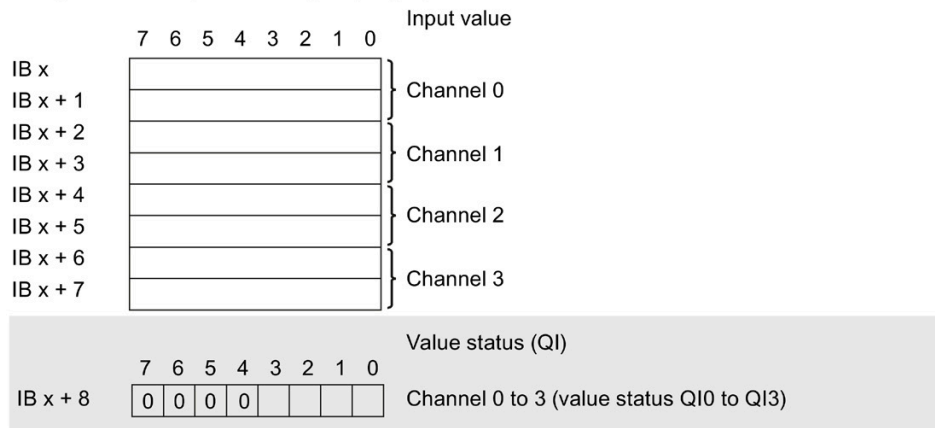
Figure 4-2 Address space of the AI 4xI 2-/4-wire ST with value status
