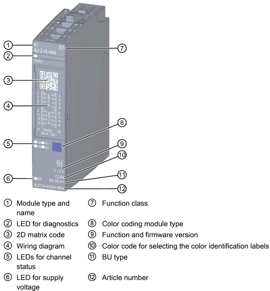
Figure 2-1 View of the module AI 4x1 2-/4-wire ST
