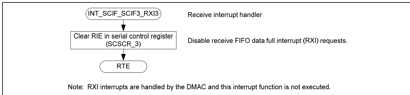
Figure 13 Processing Sequence of SCIF Receive Interrupt Handler
