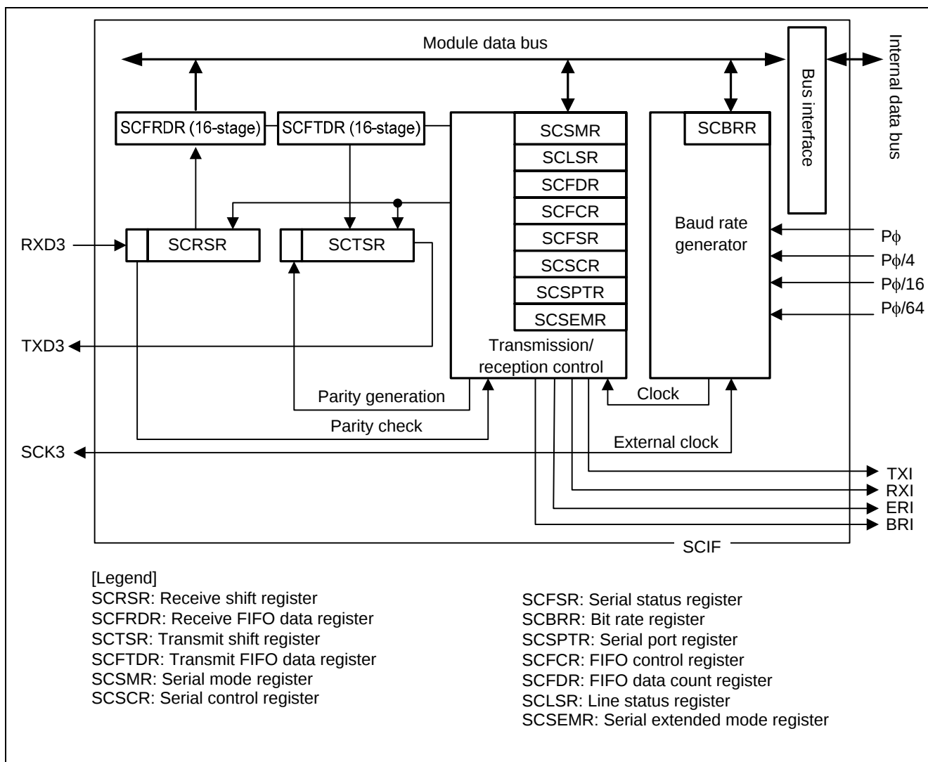
Figure 1 Block Diagram of SCIF
