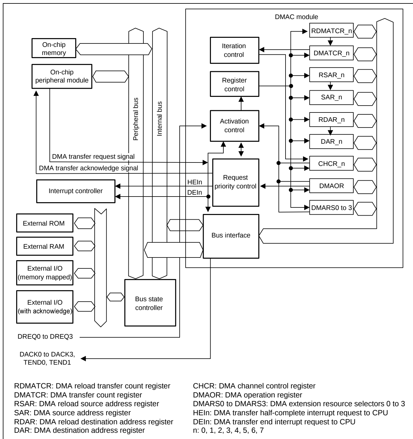
Figure 4 Block Diagram of DMAC
