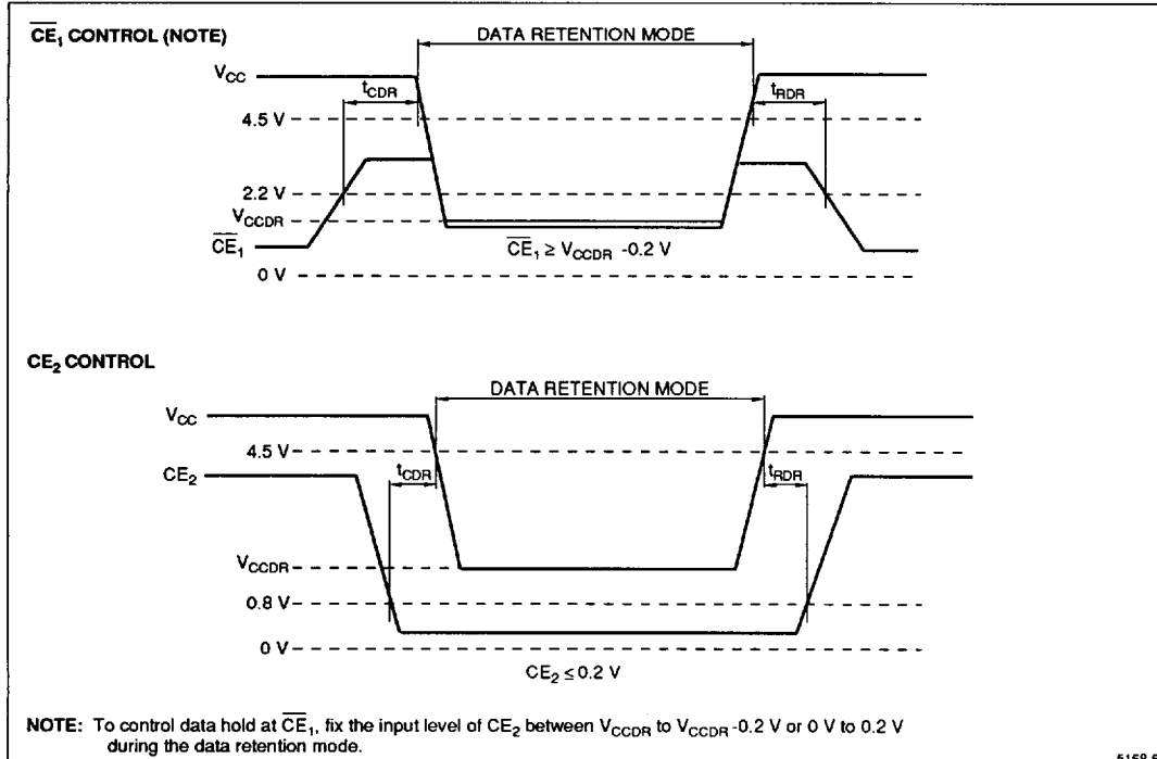
Figure 4. Low Voltage Data Retention
