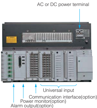
Rear panel of the stand-alone model
