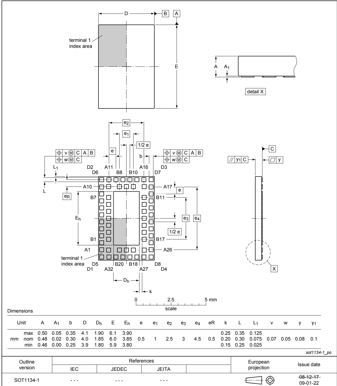
Fig. 1. Package outline HXQFN60U (SOT1134-1)
