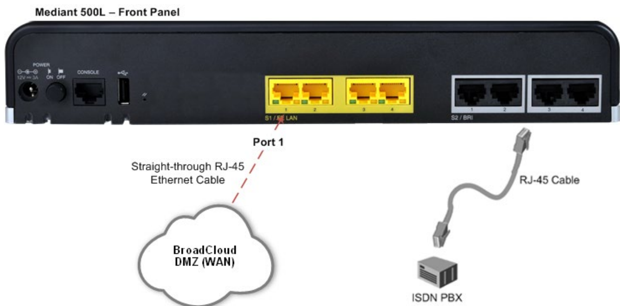
Figure 6-2: Mediant 500L BRI Media Gateway
