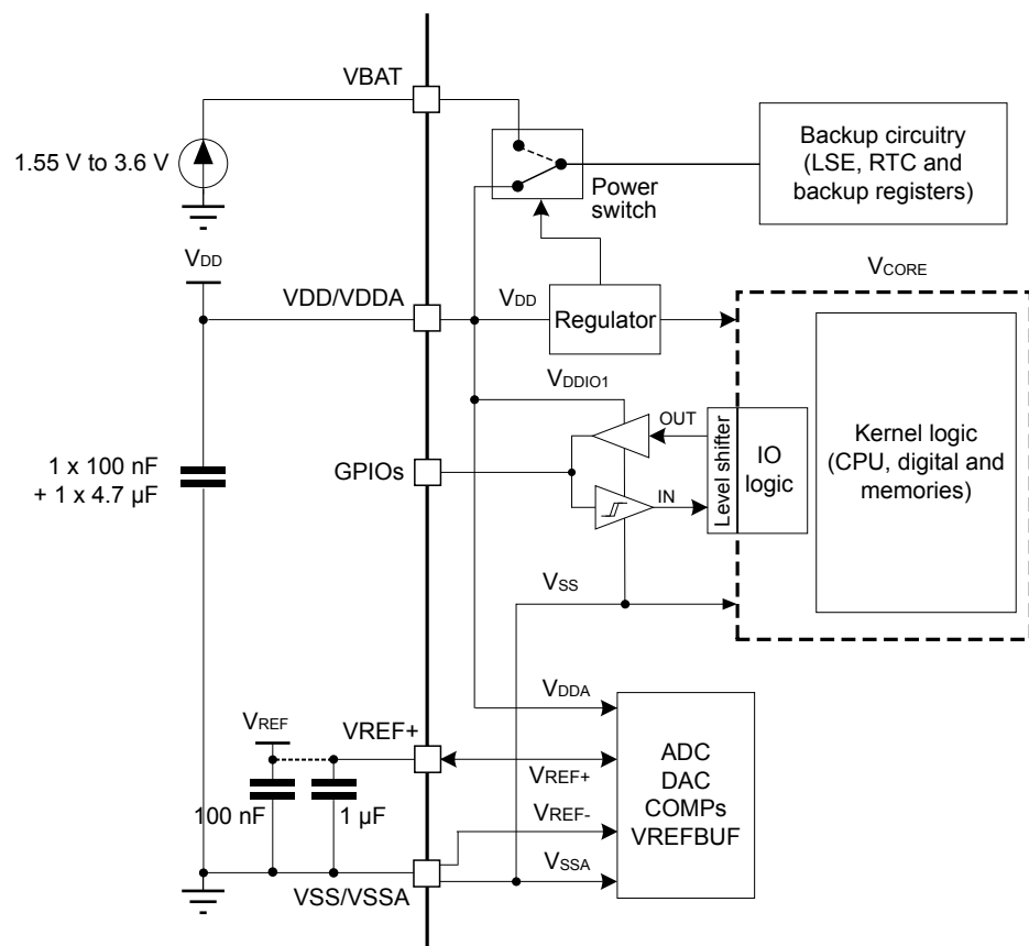
Figure 1. STM32G0 Series power supply
