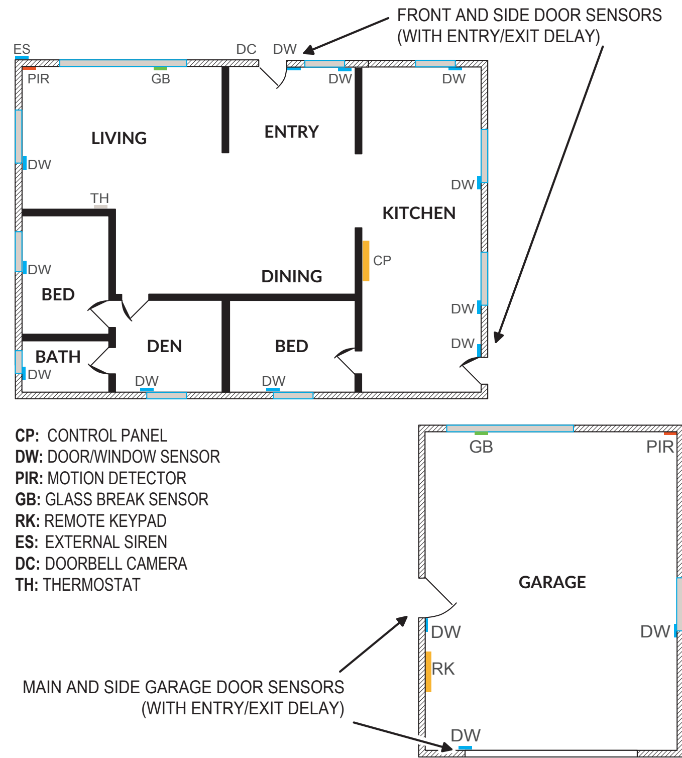
Sample Burglary Alarm Plan
