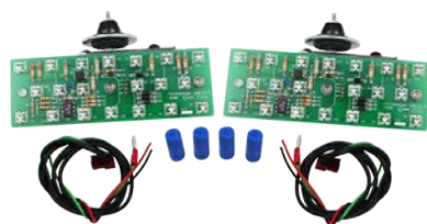
6699 '69 L.E.D. Conversion
