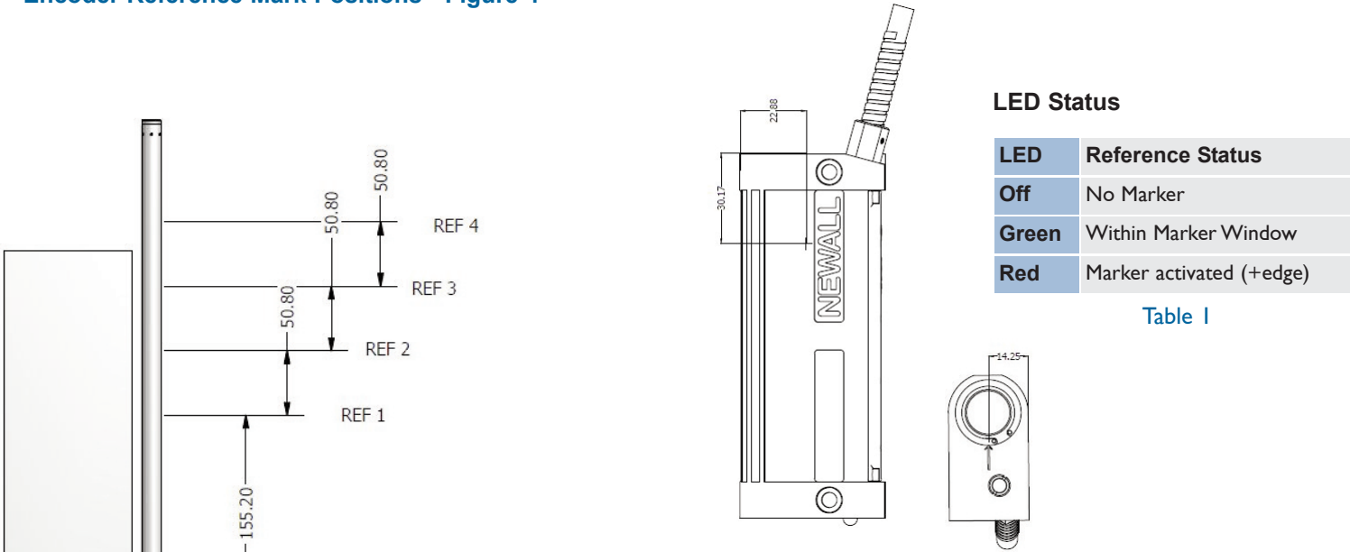
Encoder Reference Mark Positions - Figure 4
