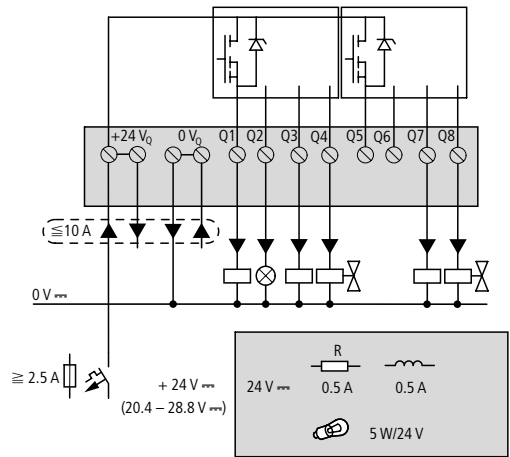
Figure 29: EZ7...-...-T.. transistor outputs
