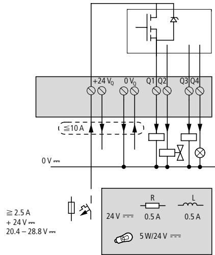
Figure 28: EZ512-...-T.. transistor outputs
