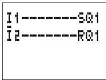
S1 make contact at I1 S2 break contact at I2
