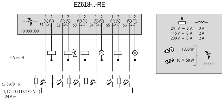
Figure 27: EZ618-..-RE.. relay outputs
