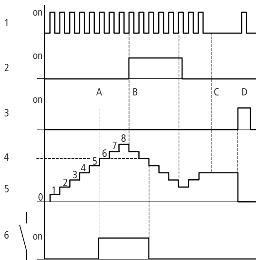
Figure 54: Signal diagram
