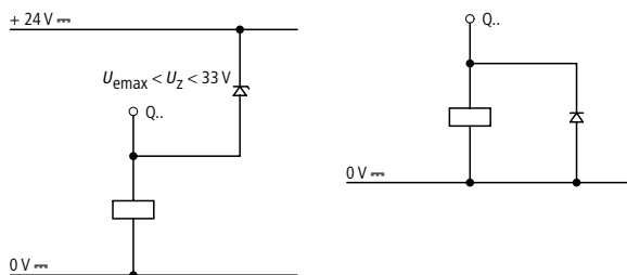
Figure 31: Inductive load with suppressor circuit
