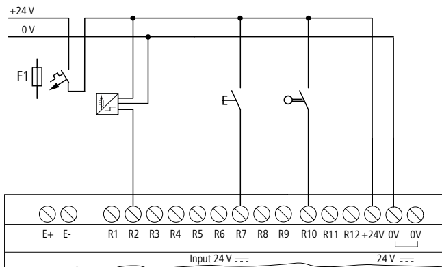
Figure 16: Connecting EZ...-DC-E digital inputs
