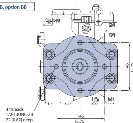
View "X"
