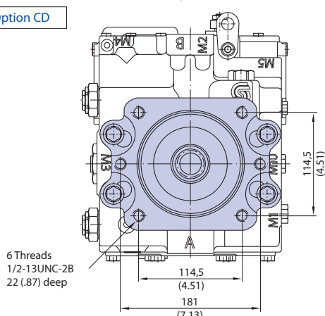
View "X"
