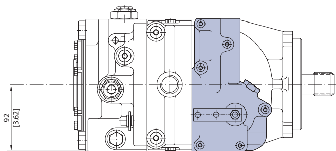
View "Y"
