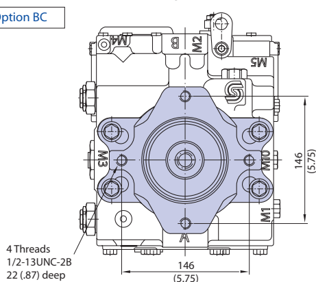
View "X"
