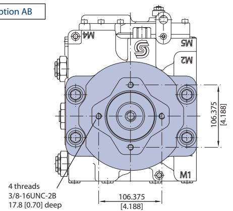
View "X"
