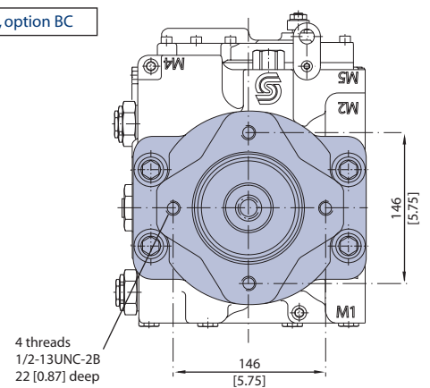
View "X"
