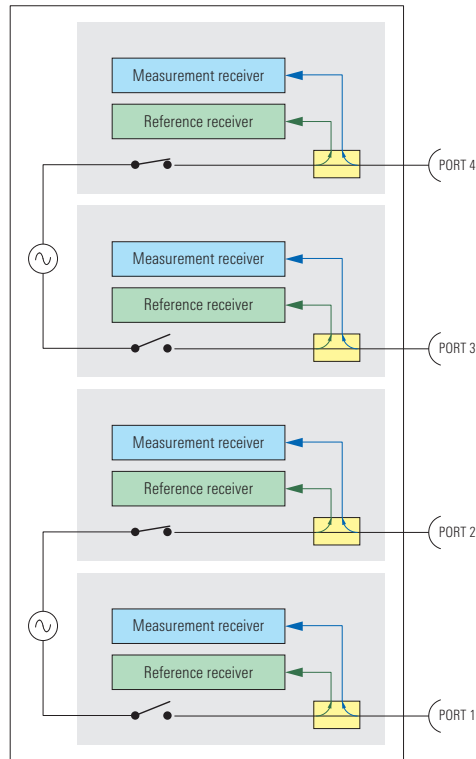
Block diagram of the R&S®ZVA8/24/40/50 four-port models
