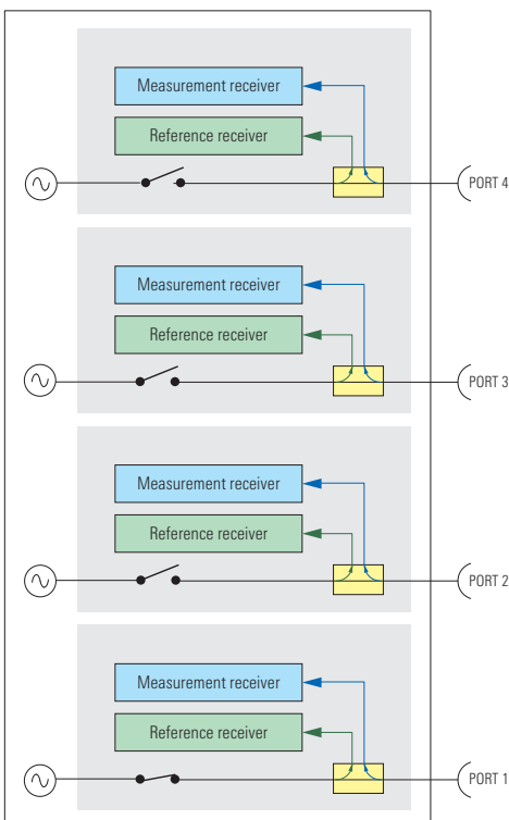
Block diagram of the R&S®ZVA67 four-port model
