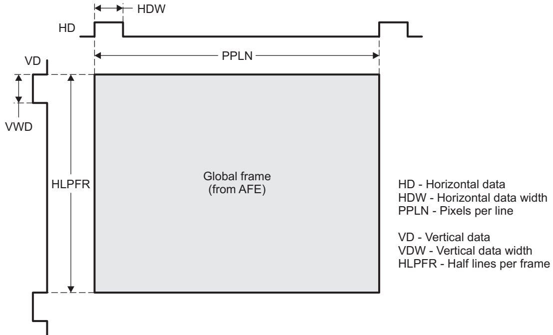
Figure 4. Raw Mode Timing Diagram
