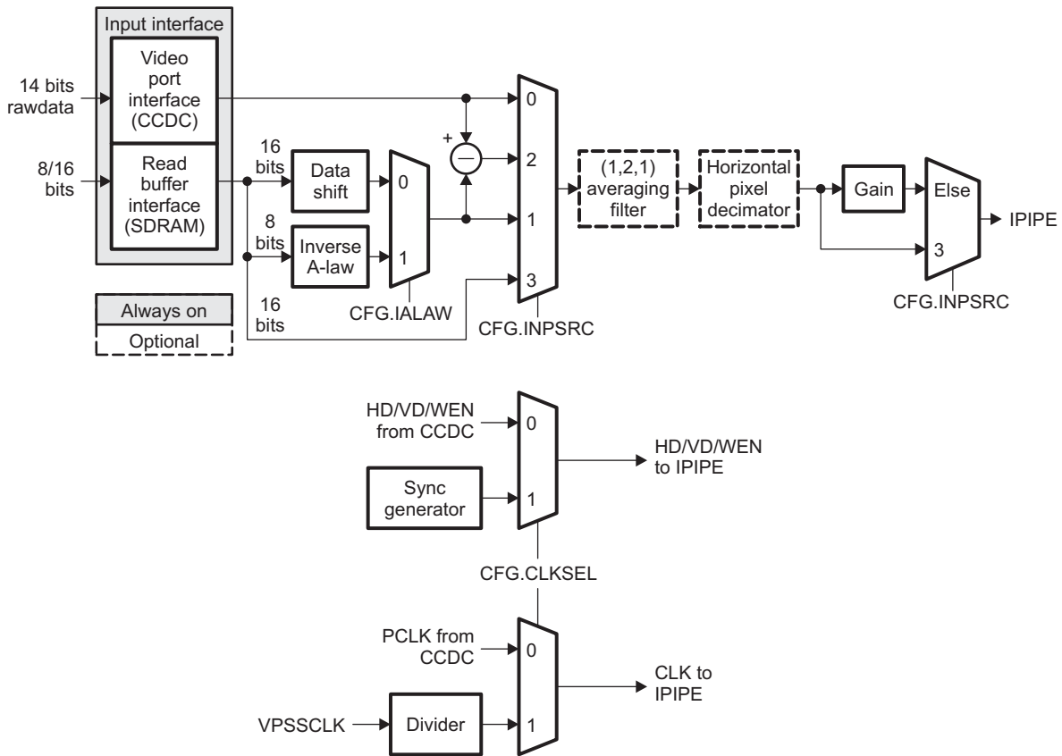
Figure 34. Image Pipe Interface Processing Flow
