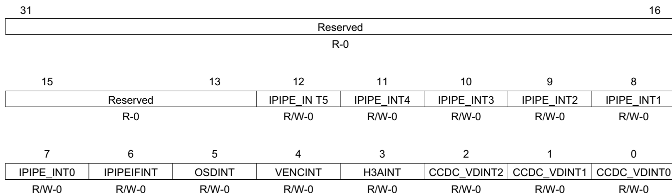
Figure 315. Interrupt Status Register (INTSTAT)
