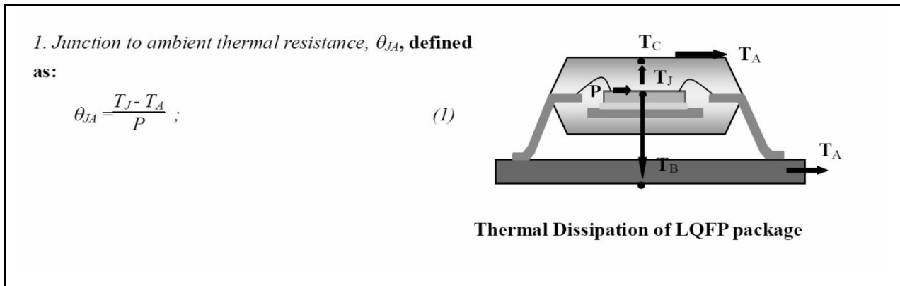
Figure 8.4-1 Junction to Ambient Thermal Resistance
