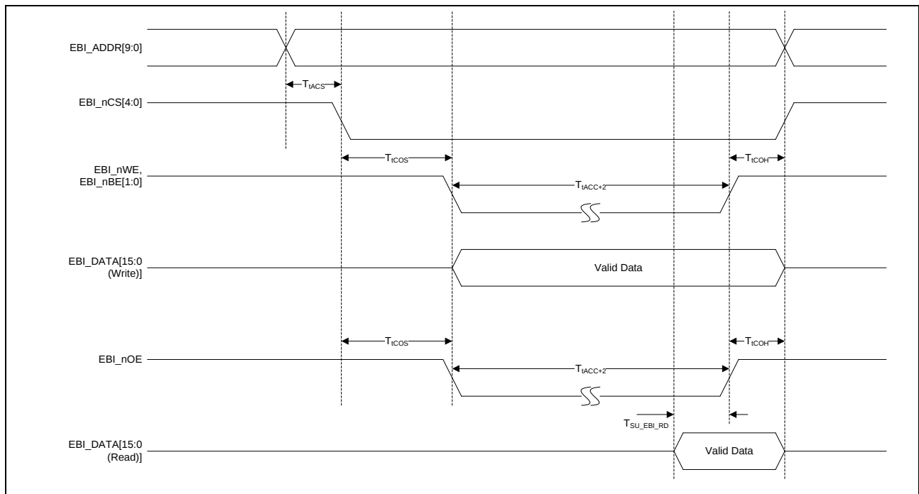
Figure 7.3-5 External Bus Interface Timing Diagram
