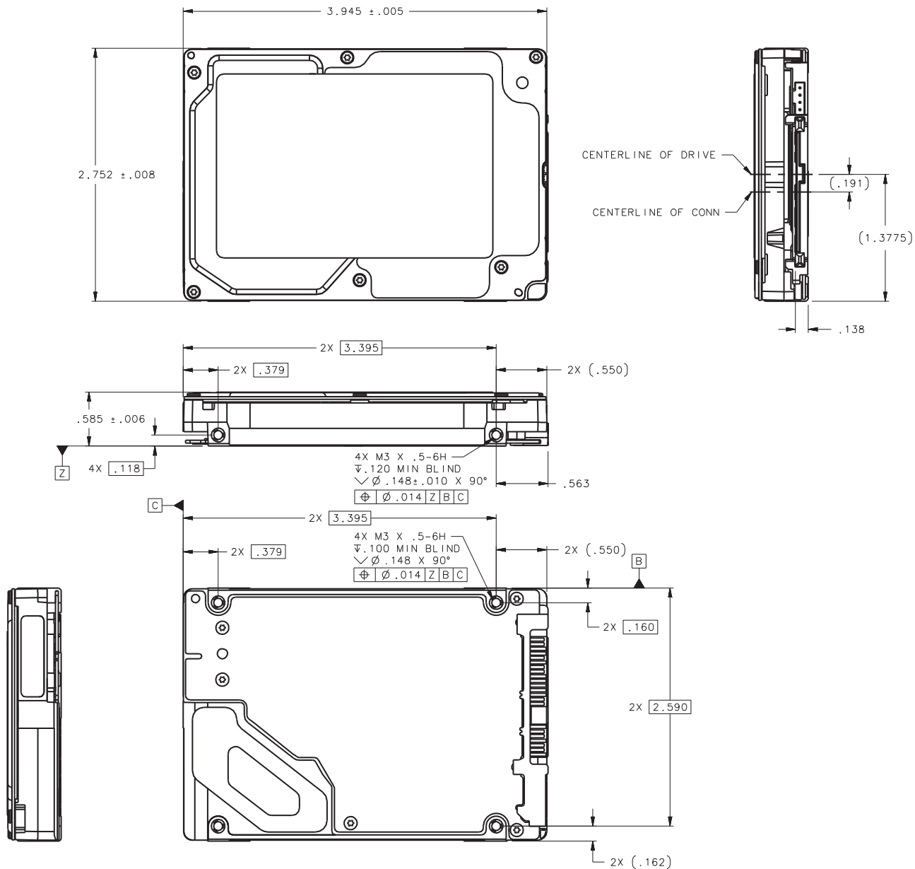
Figure 9. Dimensions
