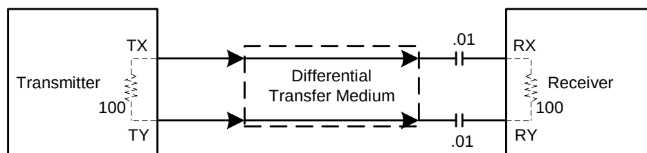
Figure 16. SAS transmitters and receivers
