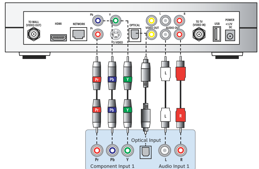
Input connectors on rear of TV
