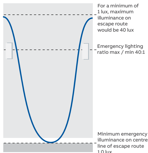
Figure 23: Uniformity requirement along escape routes
