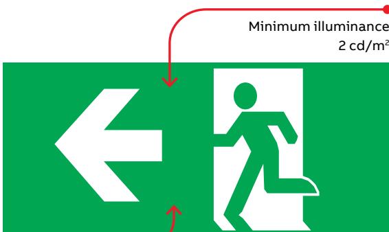
Figure 16: Exit sign formats and minimum illuminance/contrast ratios for emergency exit signs
