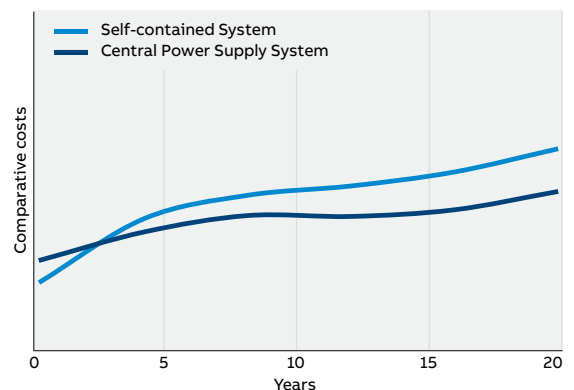
Figure 5: Comparative cost of purchasing and running self-contained and central power supply systems (typical case)
