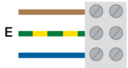
Direct slave, 3 wires +/- or AC supply: (usually AC/DC 24 V, 50 V, 110 V or 220 - 240 Vac, see Section 3.6)
