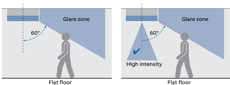
Figure 31: Disability glare at floor level
