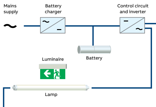
Figure 4: Schematic of a self-contained emergency luminaire
