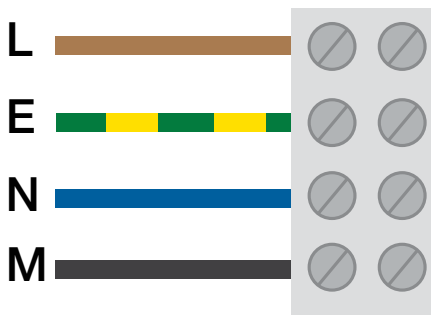
Maintained, 4 wires: Permanent live (L), Earth (E), Neutral (N), Switched live (M)
