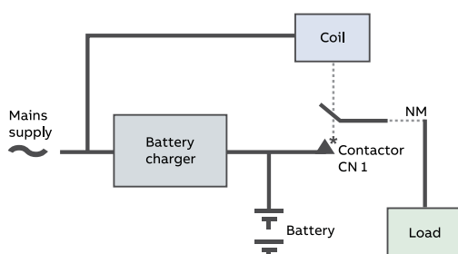
Figure 7: Non-Maintained DC system
