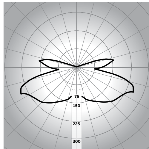
Figure 41: Luminaire relative intensity (cd/1000 lm)
