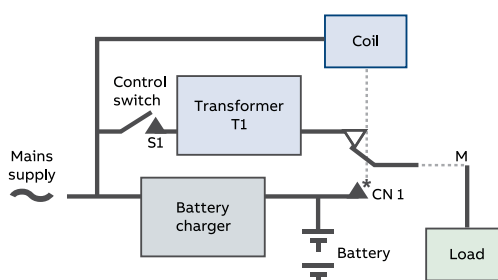
Figure 8: Maintained DC system
