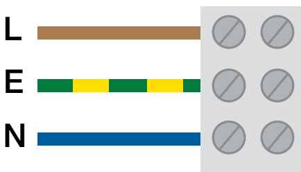
Non-maintained, 3 wires: Permanent live (L), Earth (E), Neutral (N)
