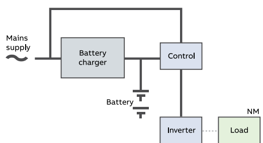
Figure 11: Non-maintained AC system
