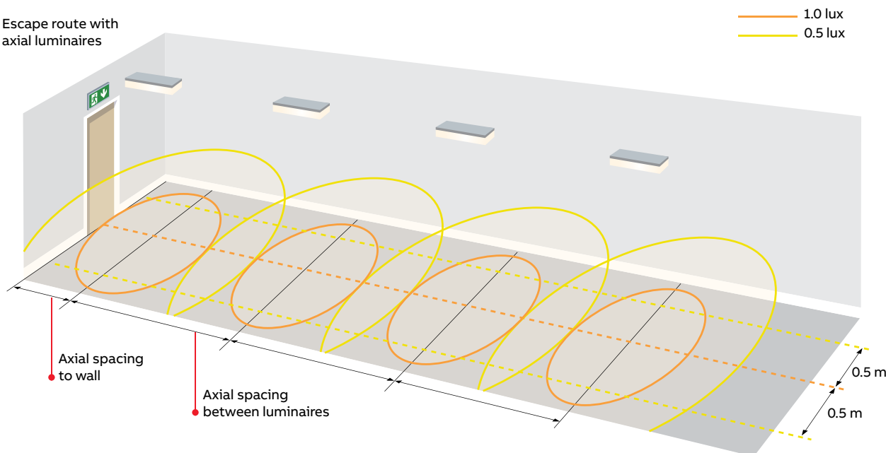
Figure 21: Axial spacing between emergency luminaires, within a 2m wide corridor
