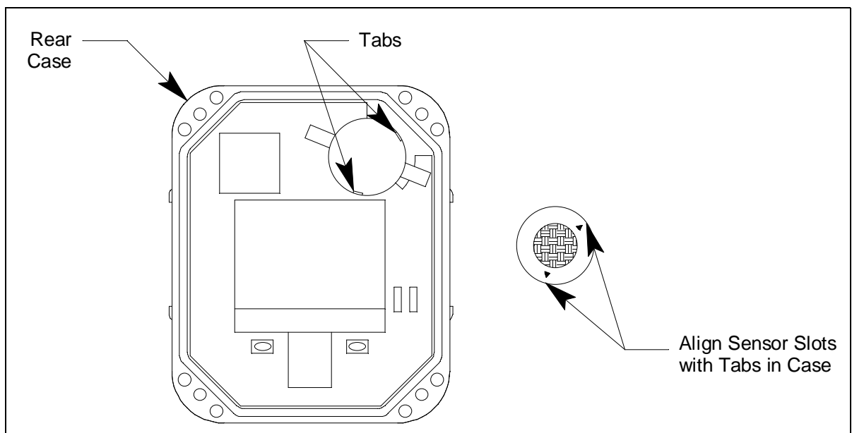
Figure 19: Sensor Location
