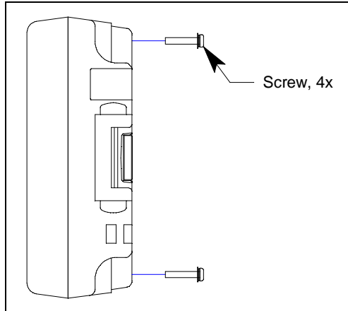
Figure 14: Unscrewing Case
