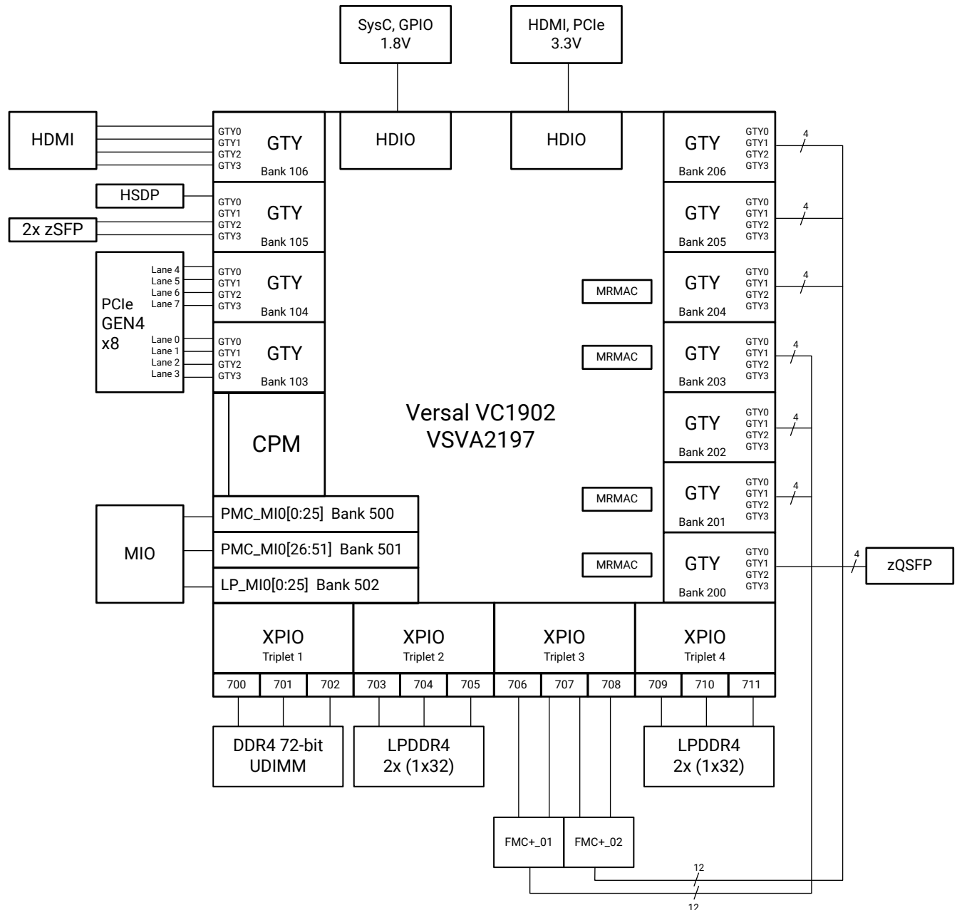
Figure 2: Block Diagram
