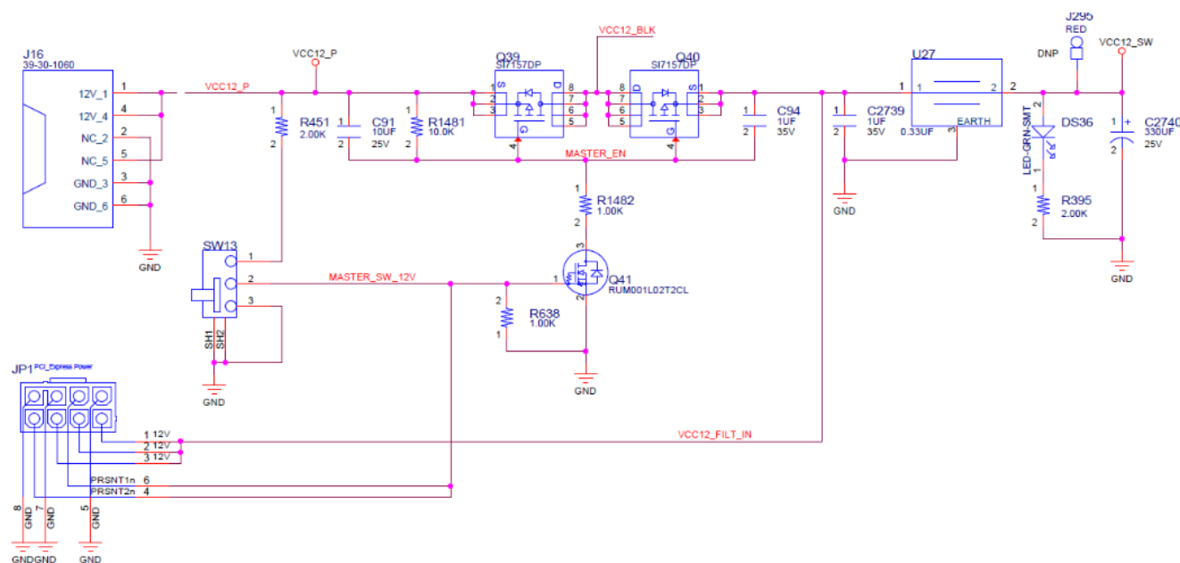
Figure 26: Power Input
