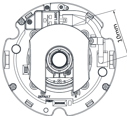
FIGURE 2-2: CONNECTING THE NETWORK CABLE
