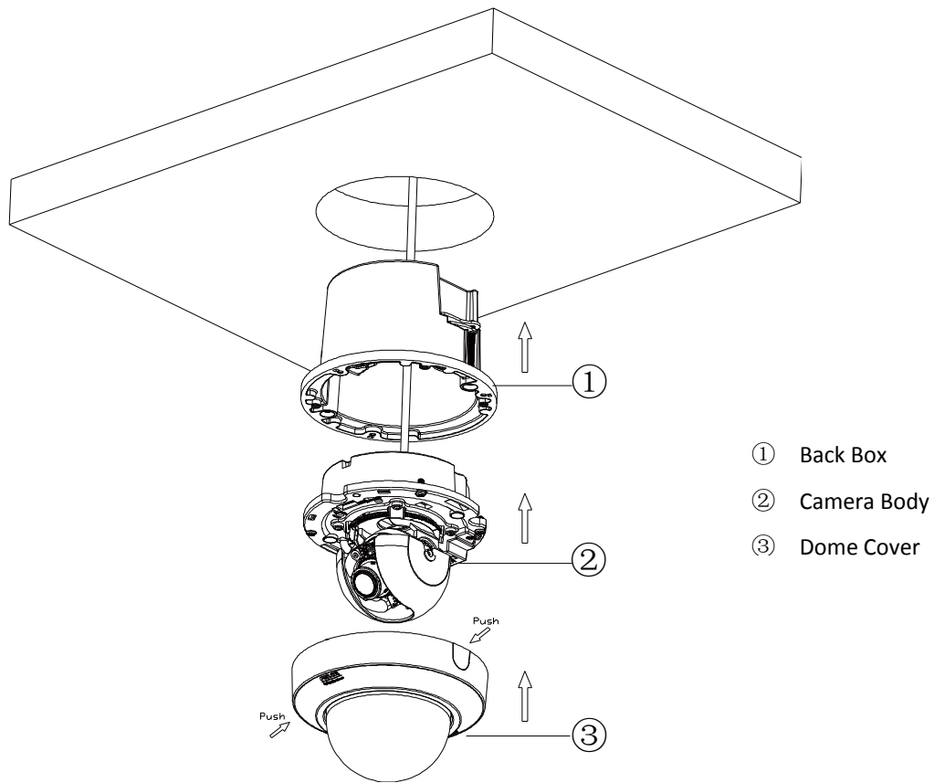
FIGURE 2-11: IN-CEILING INSTALLATION
