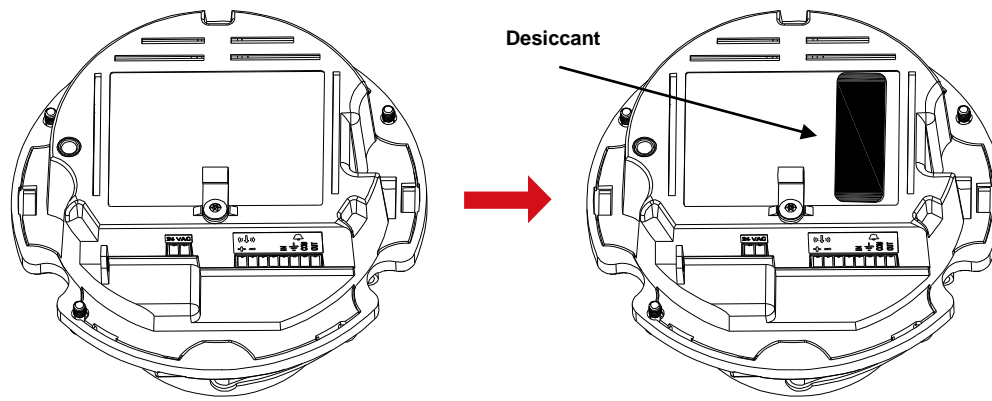
FIGURE 2-5: ATTACHING THE DESICCANT
