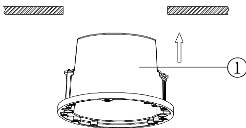
FIGURE 2-9: INSERTING THE BACK BOX
