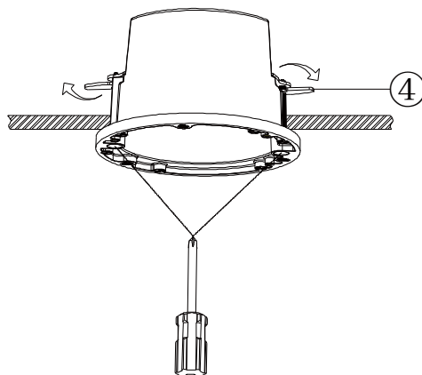
FIGURE 2-10: SECURING THE BACK BOX
