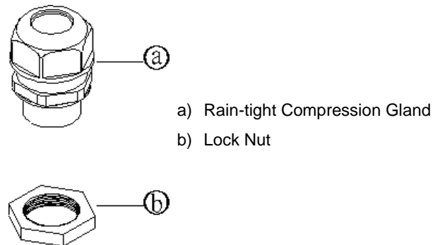
FIGURE 2-6: RAIN-TIGHT & LOCK NUT
