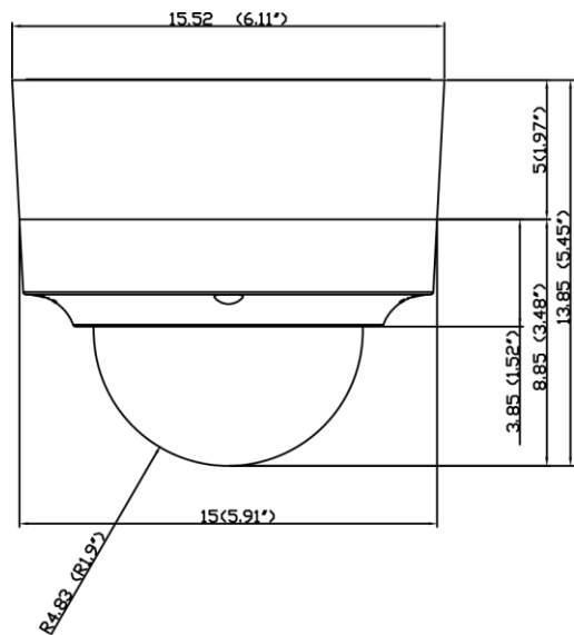
ENVIRONMENTAL DOME IN ENVIRONMENTAL SURFACE MOUNT
