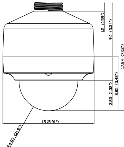
ENVIRONMENTAL DOME IN ENVIRONMENTAL PENDANT MOUNT
