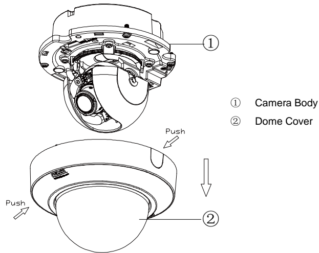
FIGURE 2-1: DISASSEMBLING THE CAMERA
