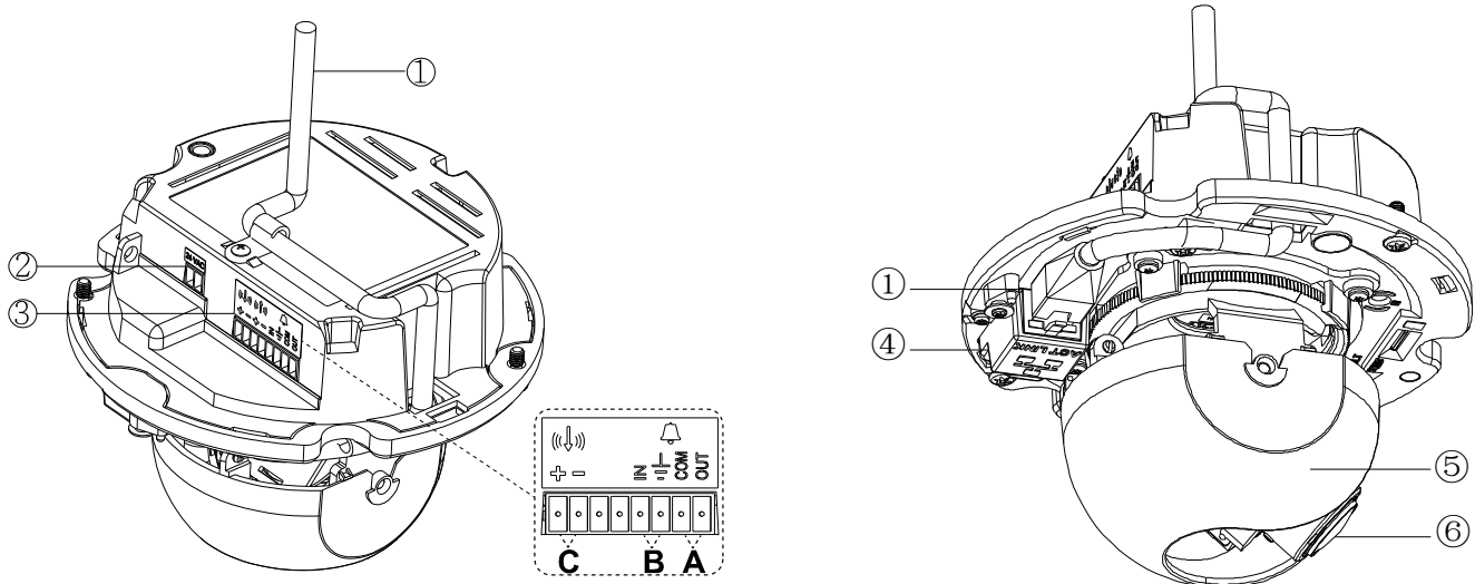
FIGURE 1-2: CAMERA CONNECTIONS AND FEATURES 1/2
