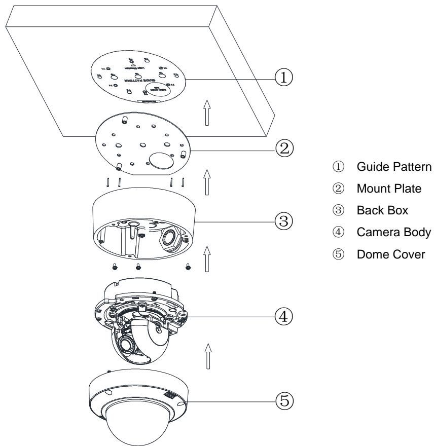
FIGURE 2-4: SURFACE INSTALLATION
