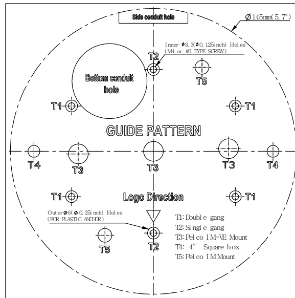
FIGURE 2-3: ATTACHING THE GUIDE PATTERN
