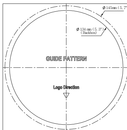
FIGURE 2-8: ATTACHING THE GUIDE PATTERN
