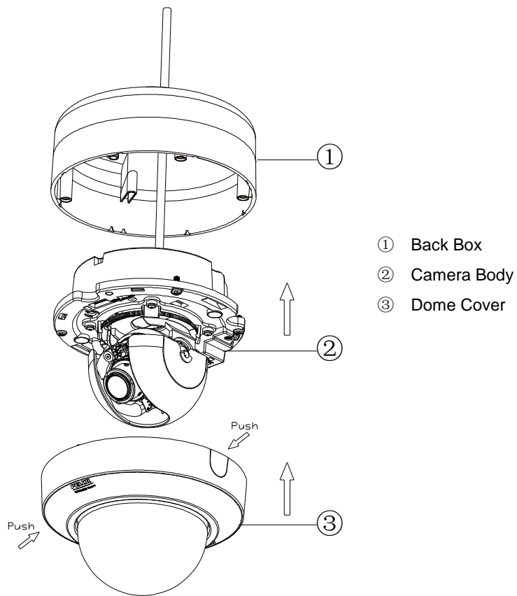
FIGURE 2-7: PENDANT INSTALLATION
