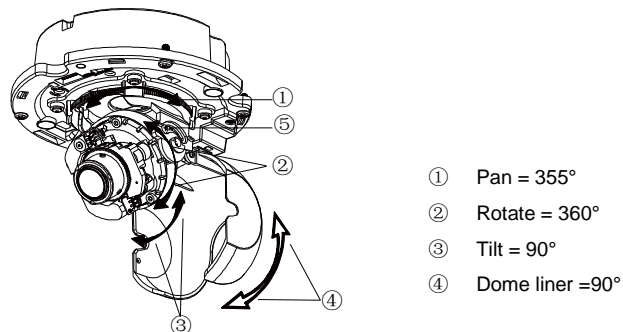
FIGURE 2-12: POSITIONING THE CAMERA
