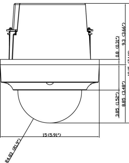
ENVIRONMENTAL DOME IN ENVIRONMENTAL CEILING MOUNT
