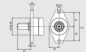
Stainless steel Flange Ordering No. 4430 2357 80
