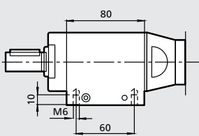
Foot Ordering No. 4430 0178 81
