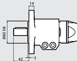
Aluminium Flange Ordering No. 4430 0569 84
