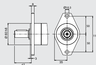
Stainless steel Flange Ordering No. 4430 2357 80
