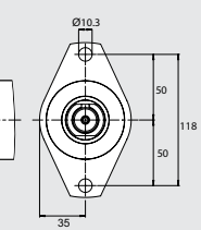
Stainless steel Flange Ordering No. 4430 2357 80
