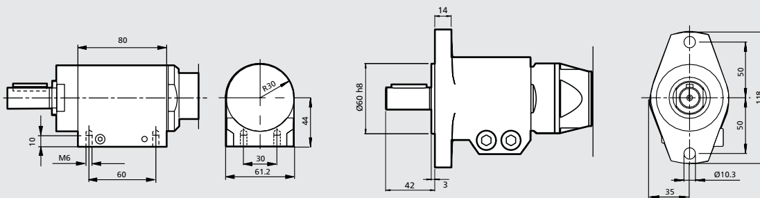
Foot Ordering No. 4430 0178 80
