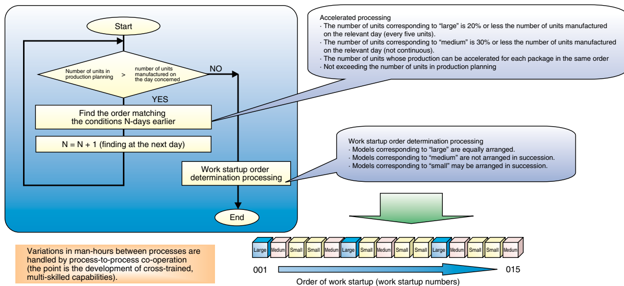
Figure 4 Example of Automatic Leveling
