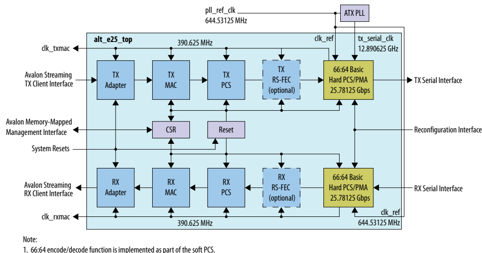
Figure 12. 25G Ethernet Intel FPGA IP Core with MAC, PCS, and PMA Clock Diagram
