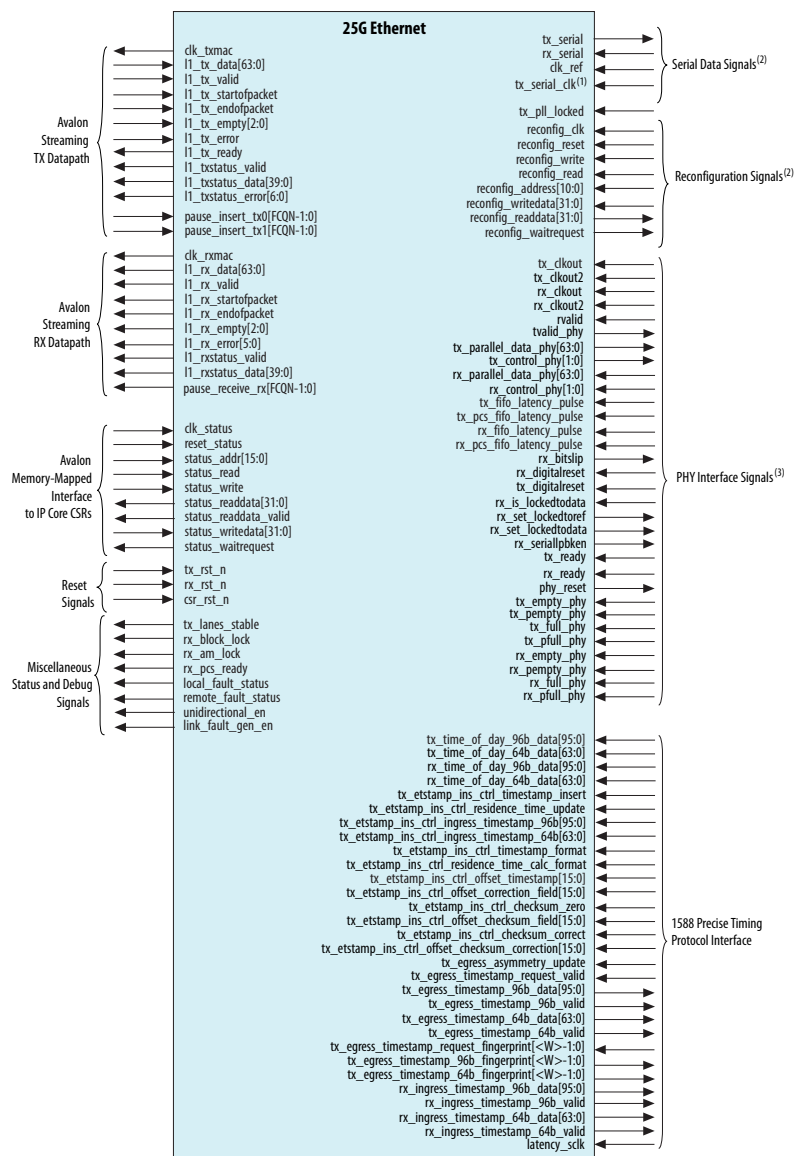
Figure 31. 25G Ethernet Intel FPGA IP Signals and Interfaces
