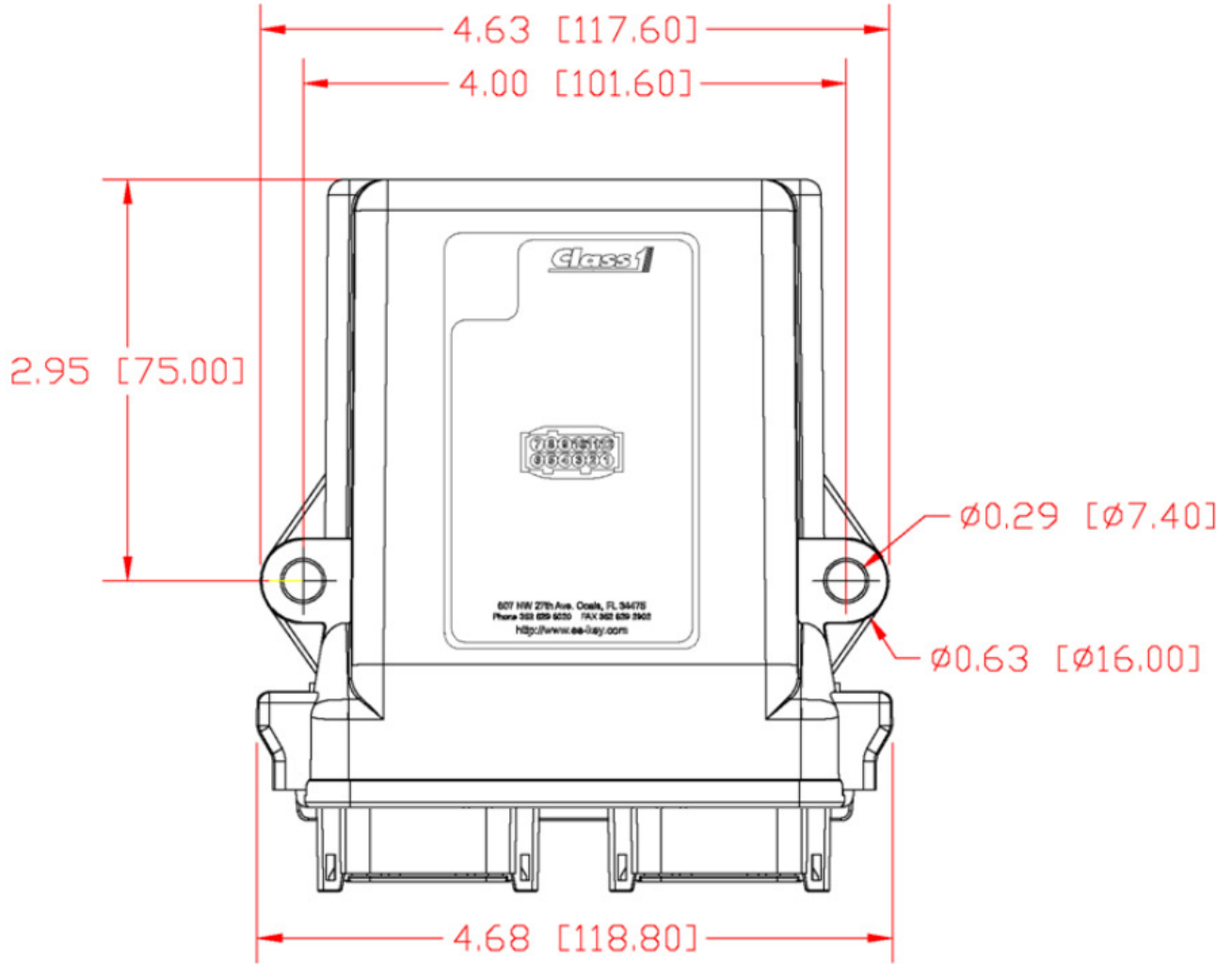
Mounting and package dimensions – inches [millimeters].
