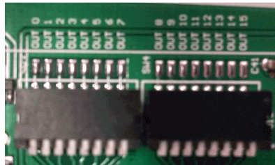
Figure 2. Output polarity selection switches.
