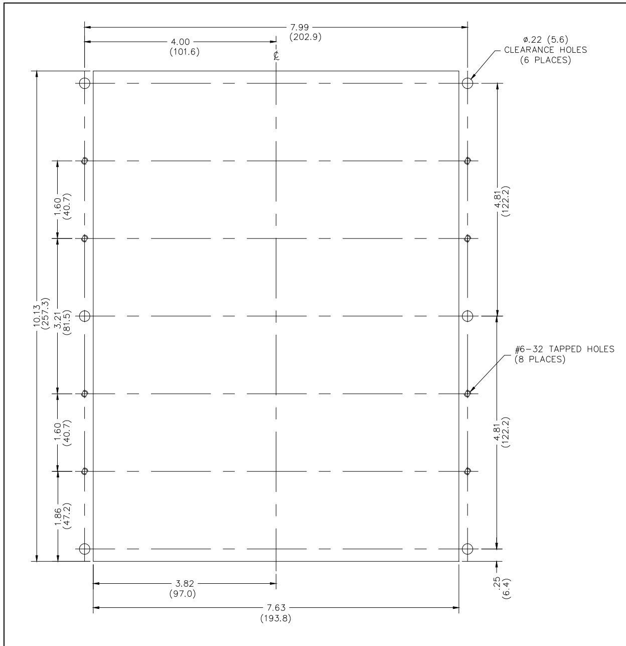
Figure 10. Cutout for Model 397-00xAD
