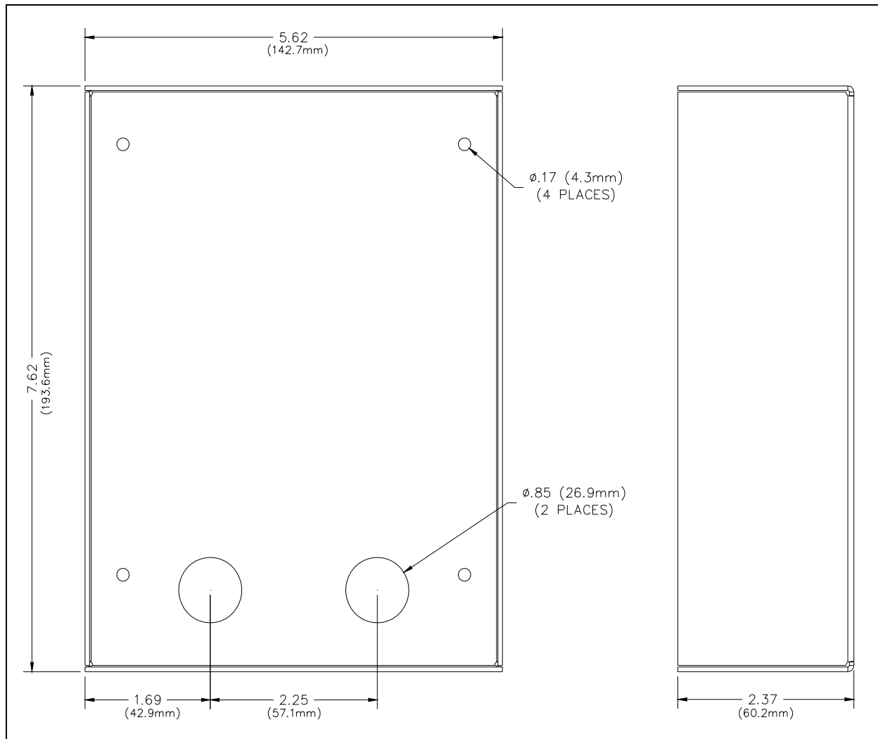
Figure 12. Model 397-001ADFS Back Box
