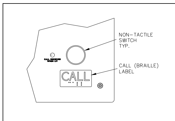
Figure 16. Extreme Cold Temperature Piezo Button (Typical)
