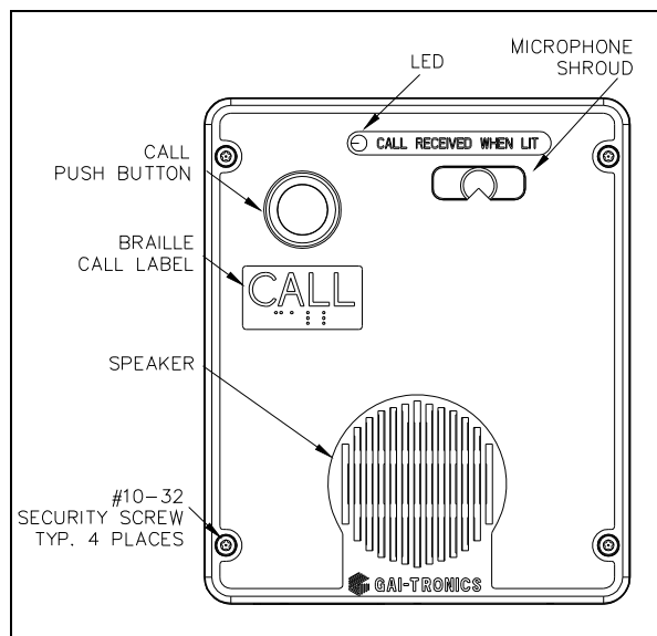
Figure 5. Model 393-001AD Telephone in a Non-Metallic Enclosure
