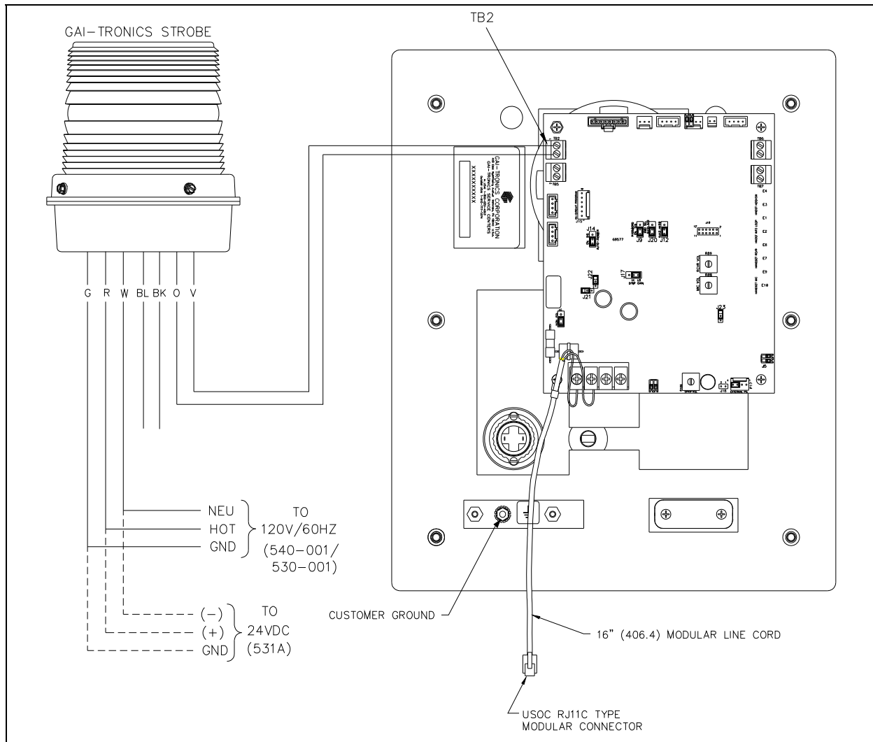
Figure 14. (Model 397-00xAD is shown as an example) Connection to Optional GAI-Tronics 540-001, 530-001, 531A Strobe
