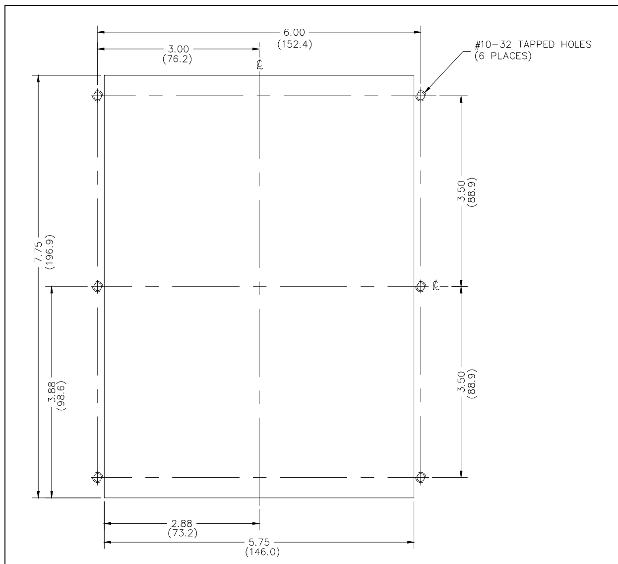
Figure 13. Cutout for Model 397-001ADFS
