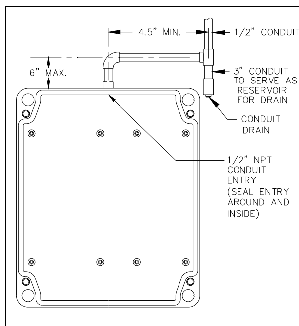
Figure 4. Top entry conduit installation details for metallic enclosures (NOT recommended)
