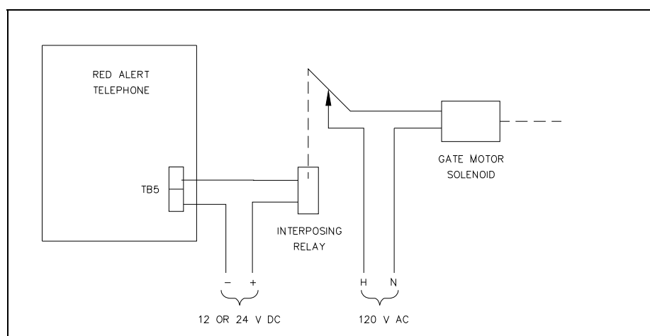
Figure 17. Example of RED ALERT® Telephone Installed for Gate Operation
