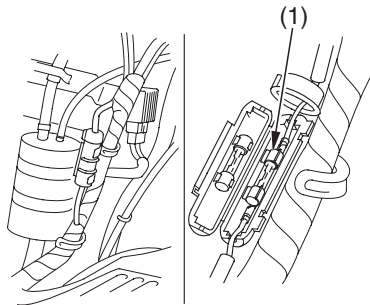
(1) main fuse
