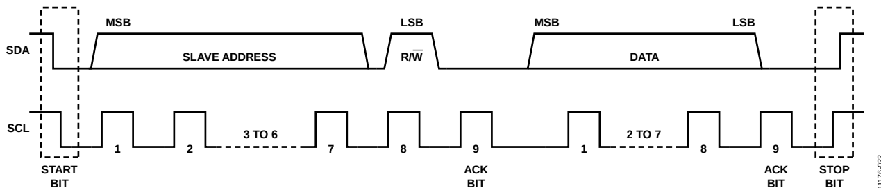
Figure 20. Typical I 2 C Transfer Sequence
