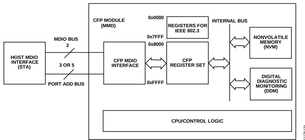
Figure 36. CFP Management Interface Architecture
