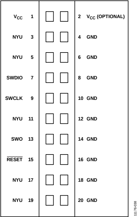
Figure 41. SWD 20-Pin Connector Pinout
