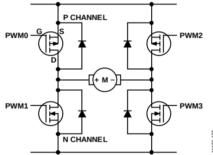
Figure 35. Example H-Bridge Configuration
