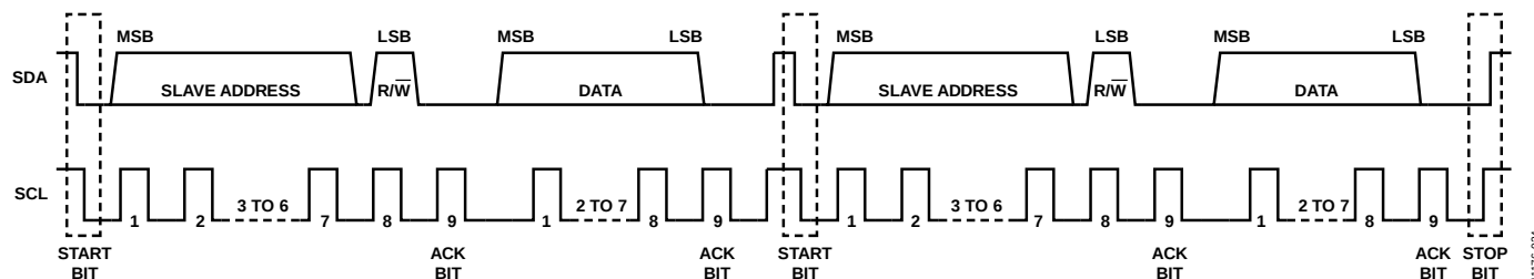
Figure 22. I²C Repeated Start Sequence
