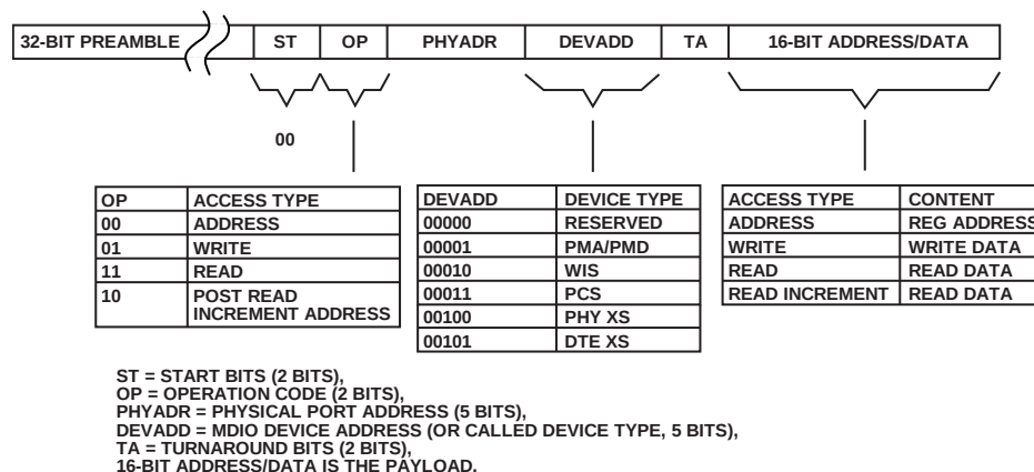
Figure 37. MDIO Frame Structure
