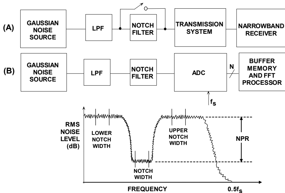
Figure 1: Noise Power Ratio (NPR) Measurements
