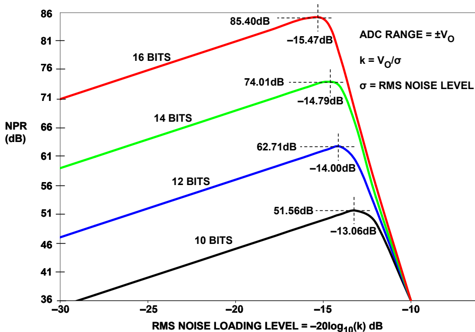
Figure 2: Theoretical NPR for 10, 12, 14, and 16-bit ADCs
