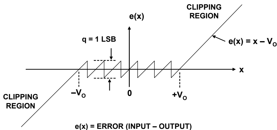
Figure 3: Ideal ADC Error Waveform
