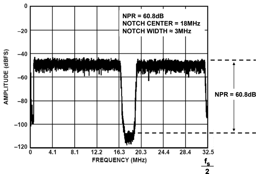
Figure 5: AD9229 12-bit, 65-MSPS ADC NPR Measures 60.8 dB (62.7 dB Theoretical)
