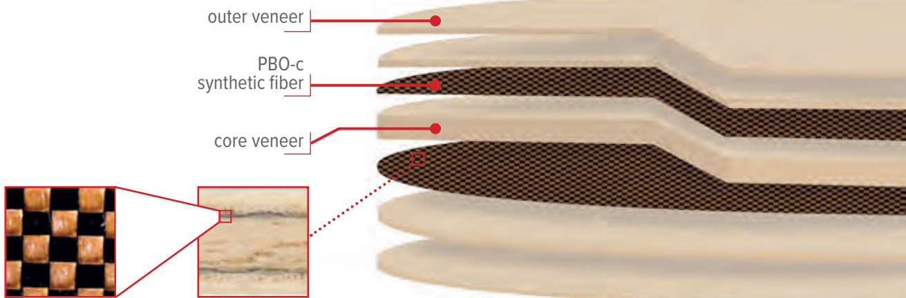
PBO-c fibers in detailed view
